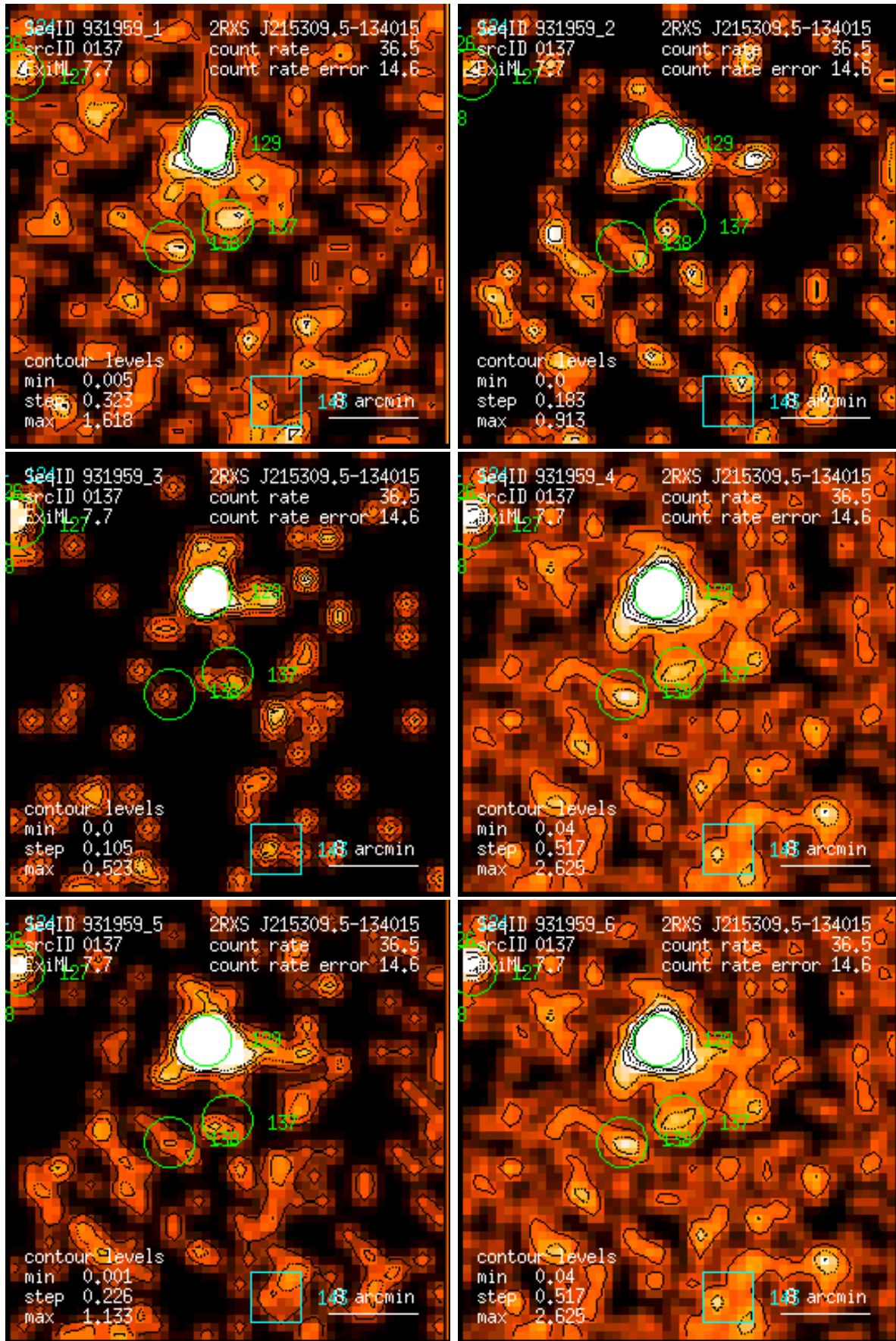
Figure 137: RASS 931959: detection 0137: band rate images, Gaussian filter: (1) PSPC channels 11 – 41, (2) 52 – 90, (3) 91 – 201, (4) 11 – 235, (5) 52 – 201, (6) 11 – 201. Broad band rates in counts/ks. Band rate contour levels in counts/ks/arcmin 2 .
