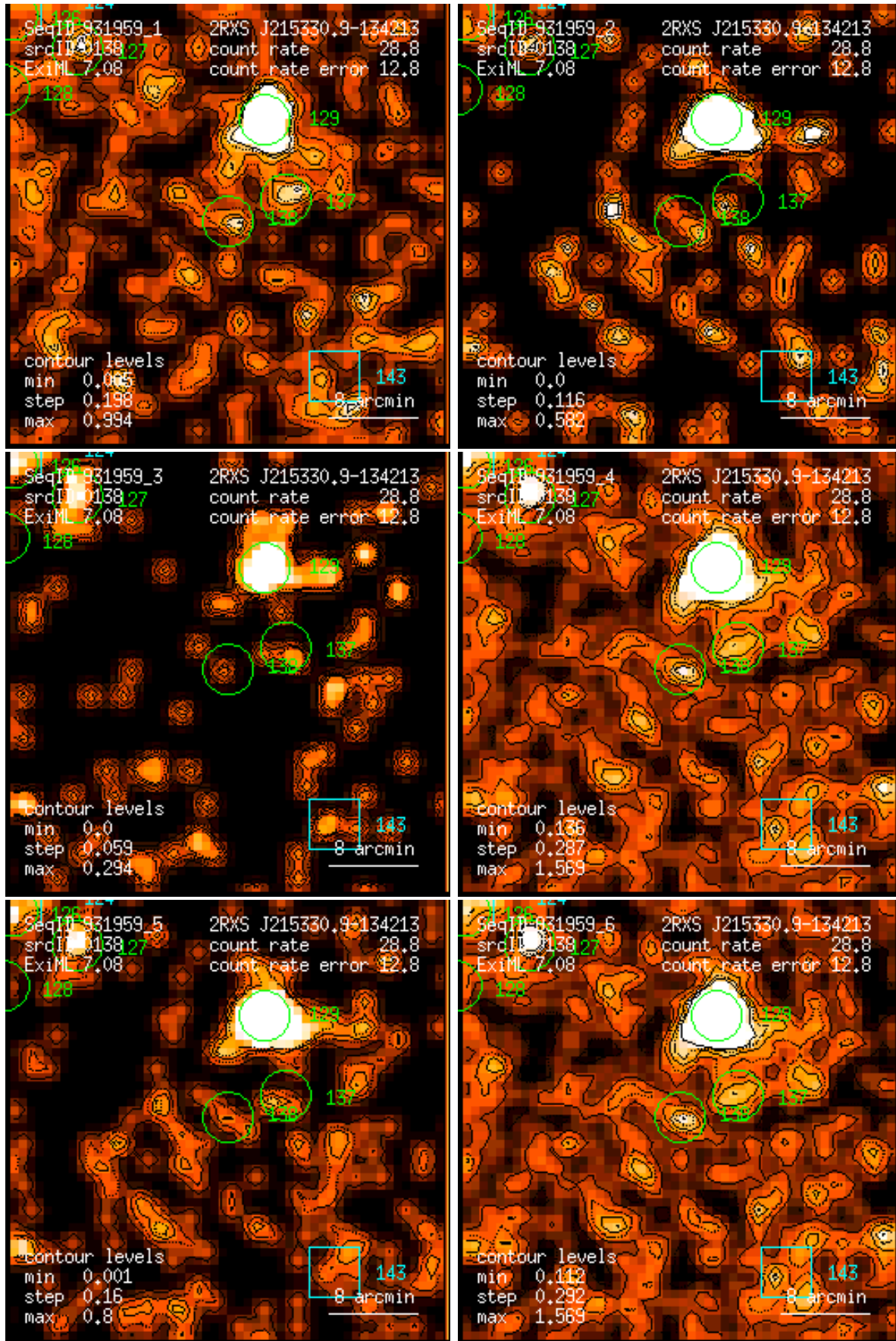
Figure 138: RASS 931959: detection 0138: band rate images, Gaussian filter: (1) PSPC channels 11 – 41, (2) 52 – 90, (3) 91 – 201, (4) 11 – 235, (5) 52 – 201, (6) 11 – 201. Broad band rates in counts/ks. Band rate contour levels in counts/ks/arcmin 2 .
