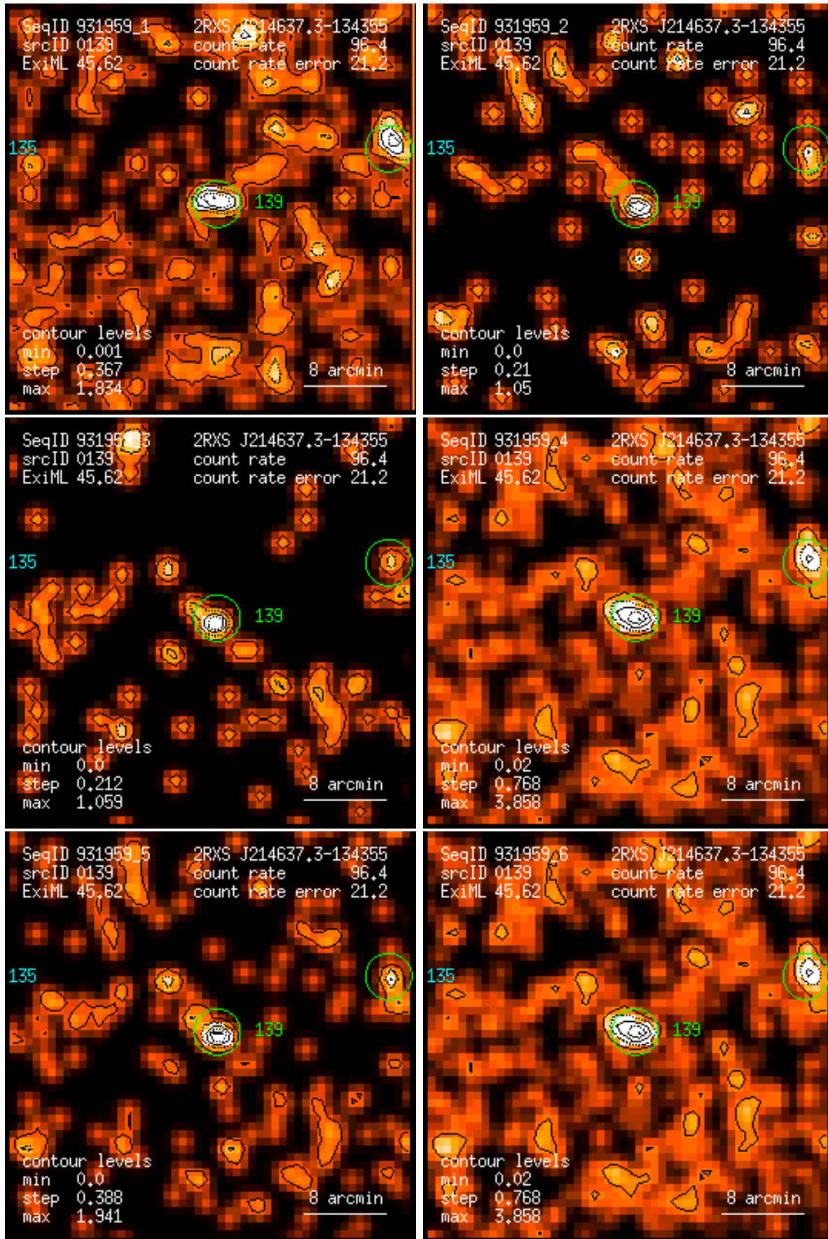
Figure 139: RASS 931959: detection 0139: band rate images, Gaussian filter: (1) PSPC channels 11 – 41, (2) 52 – 90, (3) 91 – 201, (4) 11 – 235, (5) 52 – 201, (6) 11 – 201. Broad band rates in counts/ks. Band rate contour levels in counts/ks/arcmin 2 .
