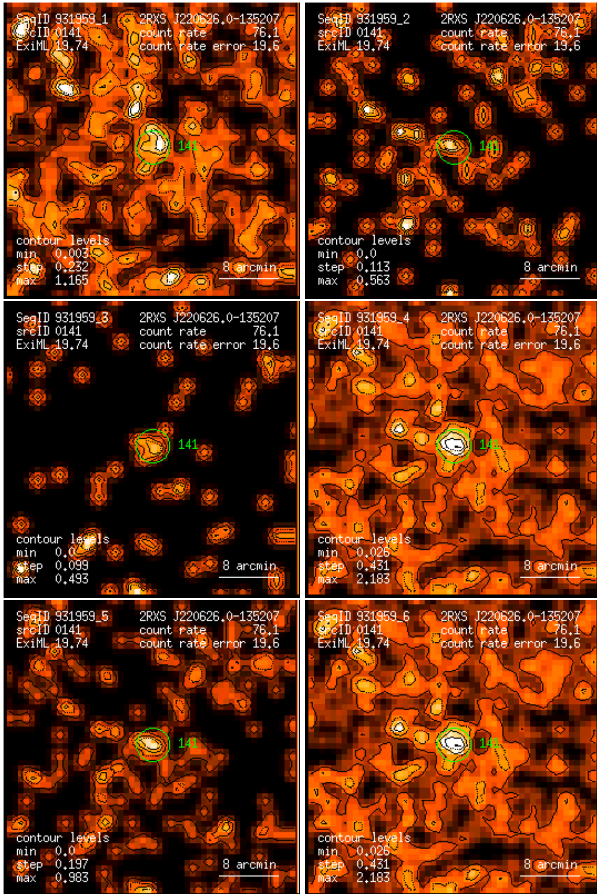
Figure 141: RASS 931959: detection 0141: band rate images, Gaussian filter: (1) PSPC channels 11 – 41, (2) 52 – 90, (3) 91 – 201, (4) 11 – 235, (5) 52 – 201, (6) 11 – 201. Broad band rates in counts/ks. Band rate contour levels in counts/ks/arcmin 2 .
