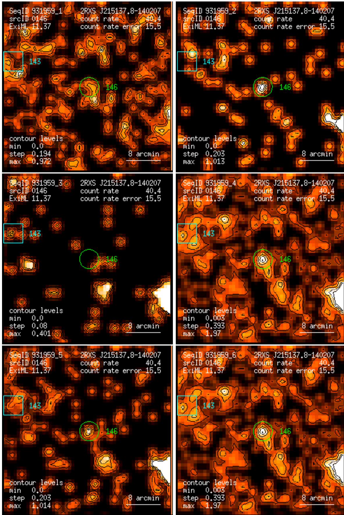
Figure 146: RASS 931959: detection 0146: band rate images, Gaussian filter: (1) PSPC channels 11 – 41, (2) 52 – 90, (3) 91 – 201, (4) 11 – 235, (5) 52 – 201, (6) 11 – 201. Broad band rates in counts/ks. Band rate contour levels in counts/ks/arcmin 2 .
