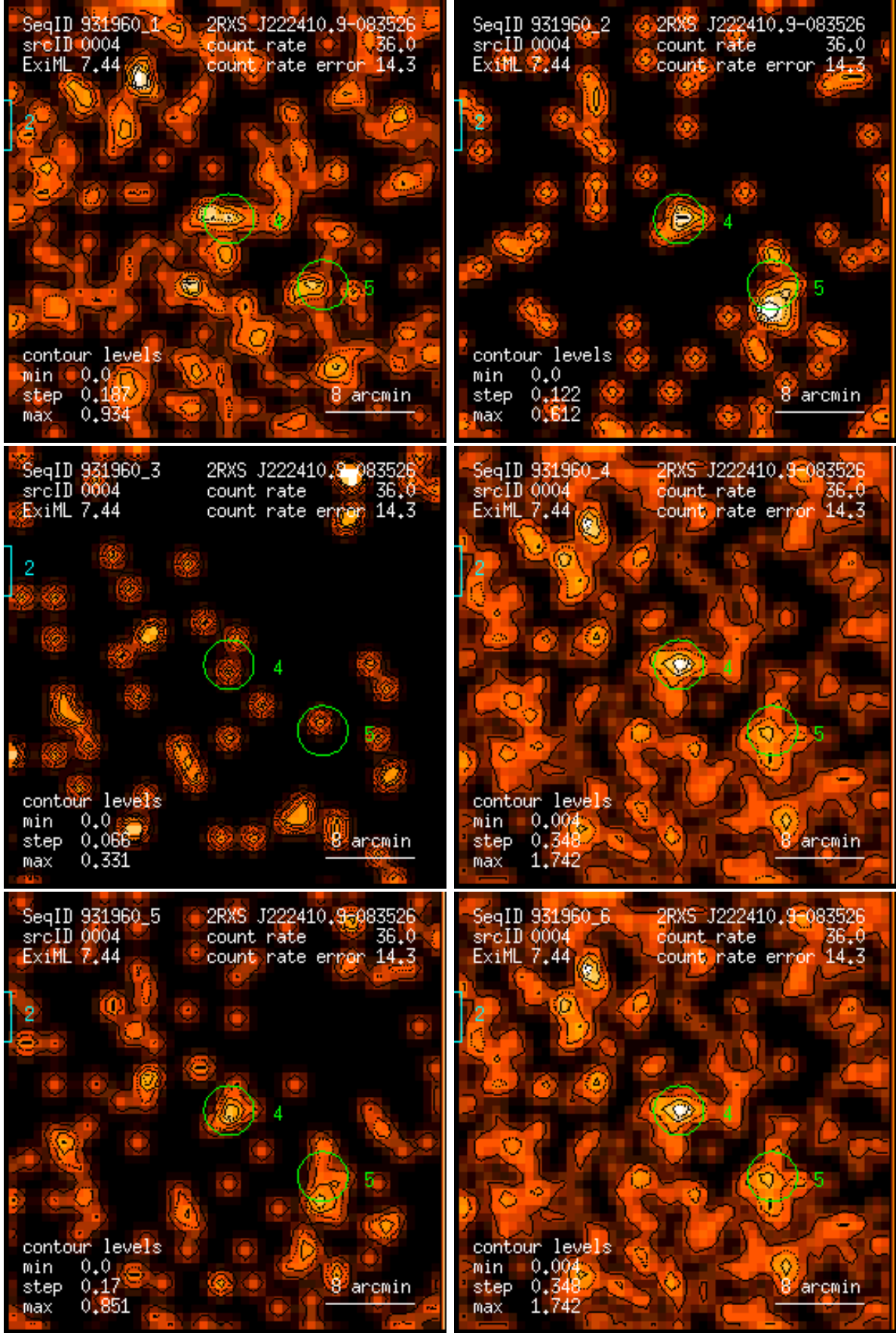
Figure 4: RASS 931960: detection 0004: band rate images, Gaussian filter: (1) PSPC channels 11 – 41, (2) 52 – 90, (3) 91 – 201, (4) 11 – 235, (5) 52 – 201, (6) 11 – 201. Broad band rates in counts/ks. Band rate contour levels in counts/ks/arcmin 2 .
