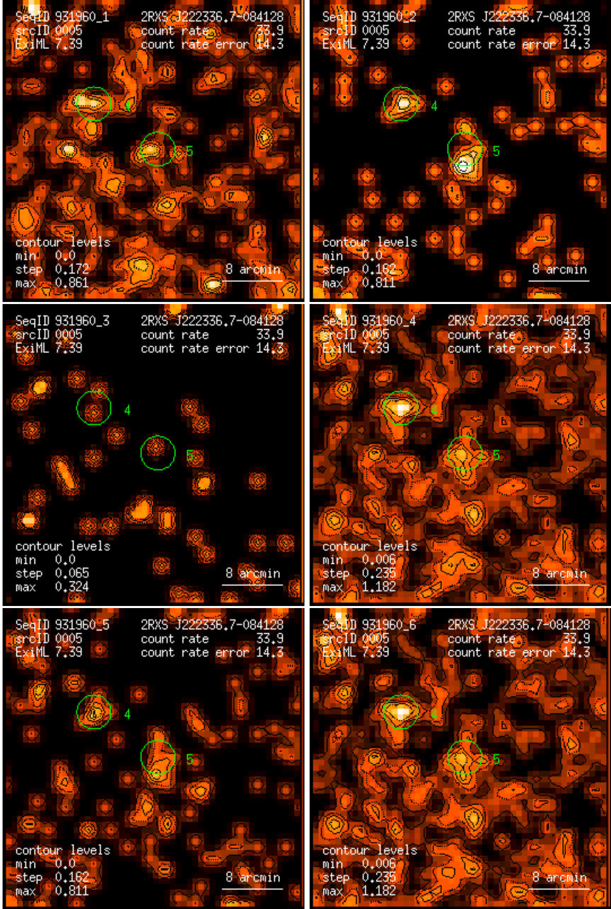
Figure 5: RASS 931960: detection 0005: band rate images, Gaussian filter: (1) PSPC channels 11 – 41, (2) 52 – 90, (3) 91 – 201, (4) 11 – 235, (5) 52 – 201, (6) 11 – 201. Broad band rates in counts/ks. Band rate contour levels in counts/ks/arcmin 2 .
