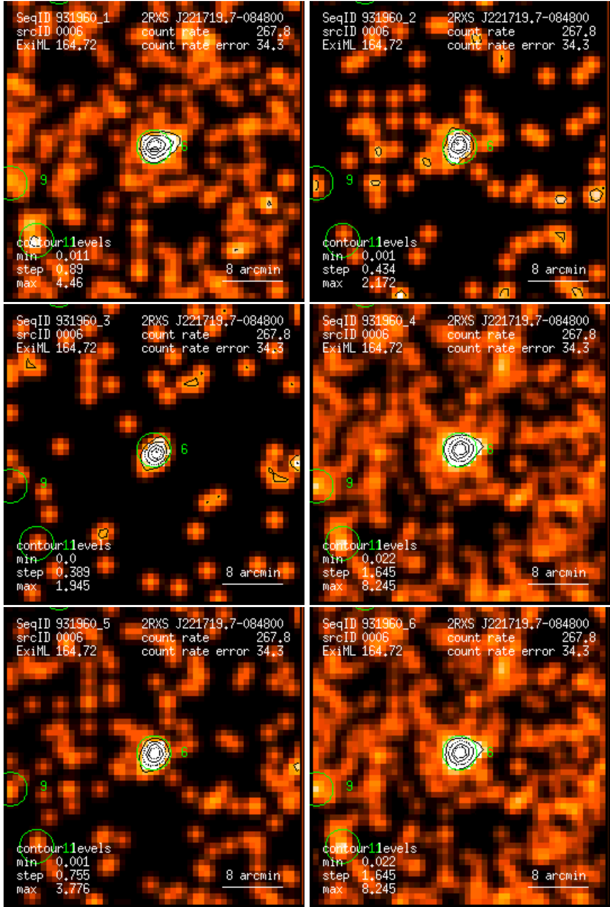
Figure 6: RASS 931960: detection 0006: band rate images, Gaussian filter: (1) PSPC channels 11 – 41, (2) 52 – 90, (3) 91 – 201, (4) 11 – 235, (5) 52 – 201, (6) 11 – 201. Broad band rates in counts/ks. Band rate contour levels in counts/ks/arcmin 2 .
