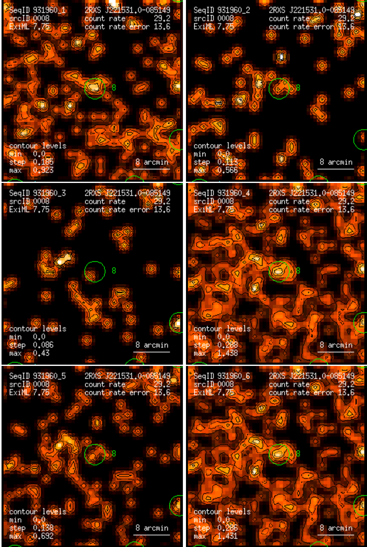
Figure 8: RASS 931960: detection 0008: band rate images, Gaussian filter: (1) PSPC channels 11 – 41, (2) 52 – 90, (3) 91 – 201, (4) 11 – 235, (5) 52 – 201, (6) 11 – 201. Broad band rates in counts/ks. Band rate contour levels in counts/ks/arcmin 2 .
