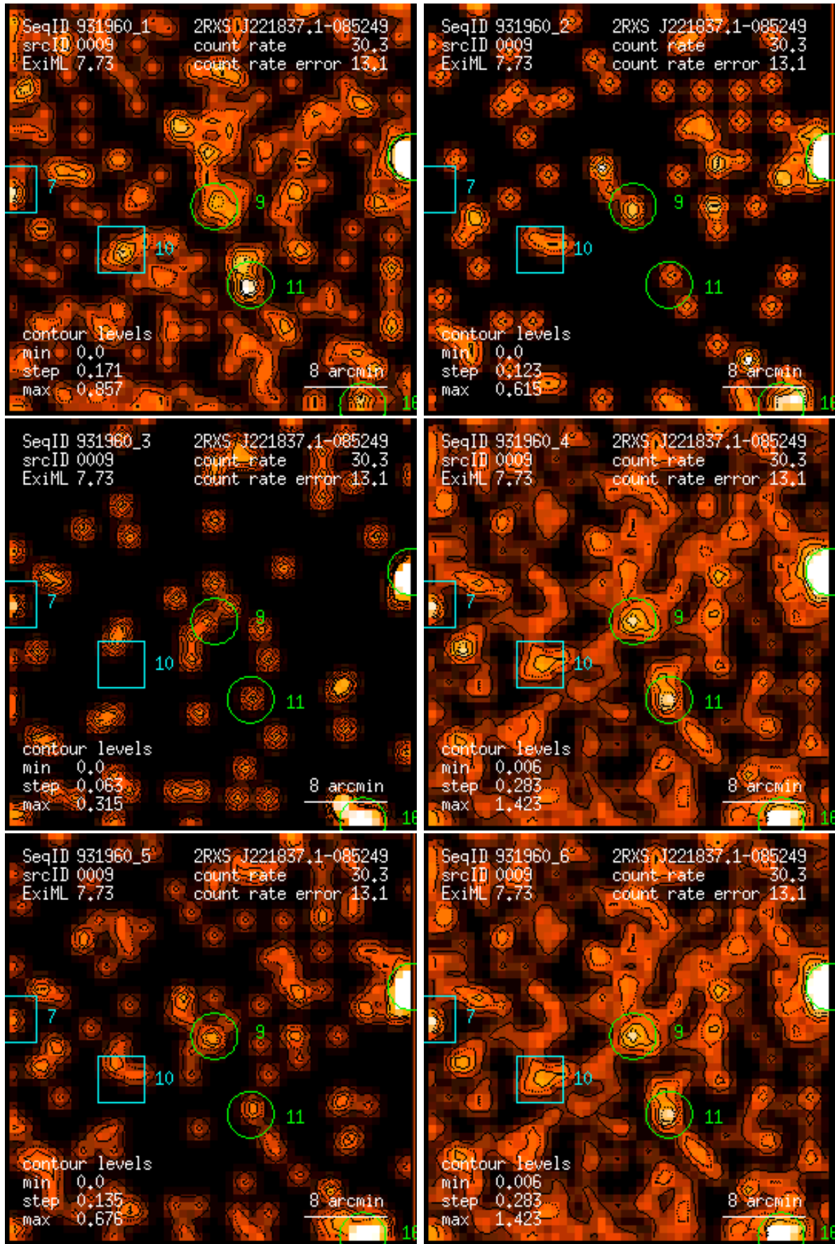
Figure 9: RASS 931960: detection 0009: band rate images, Gaussian filter: (1) PSPC channels 11 – 41, (2) 52 – 90, (3) 91 – 201, (4) 11 – 235, (5) 52 – 201, (6) 11 – 201. Broad band rates in counts/ks. Band rate contour levels in counts/ks/arcmin 2 .
