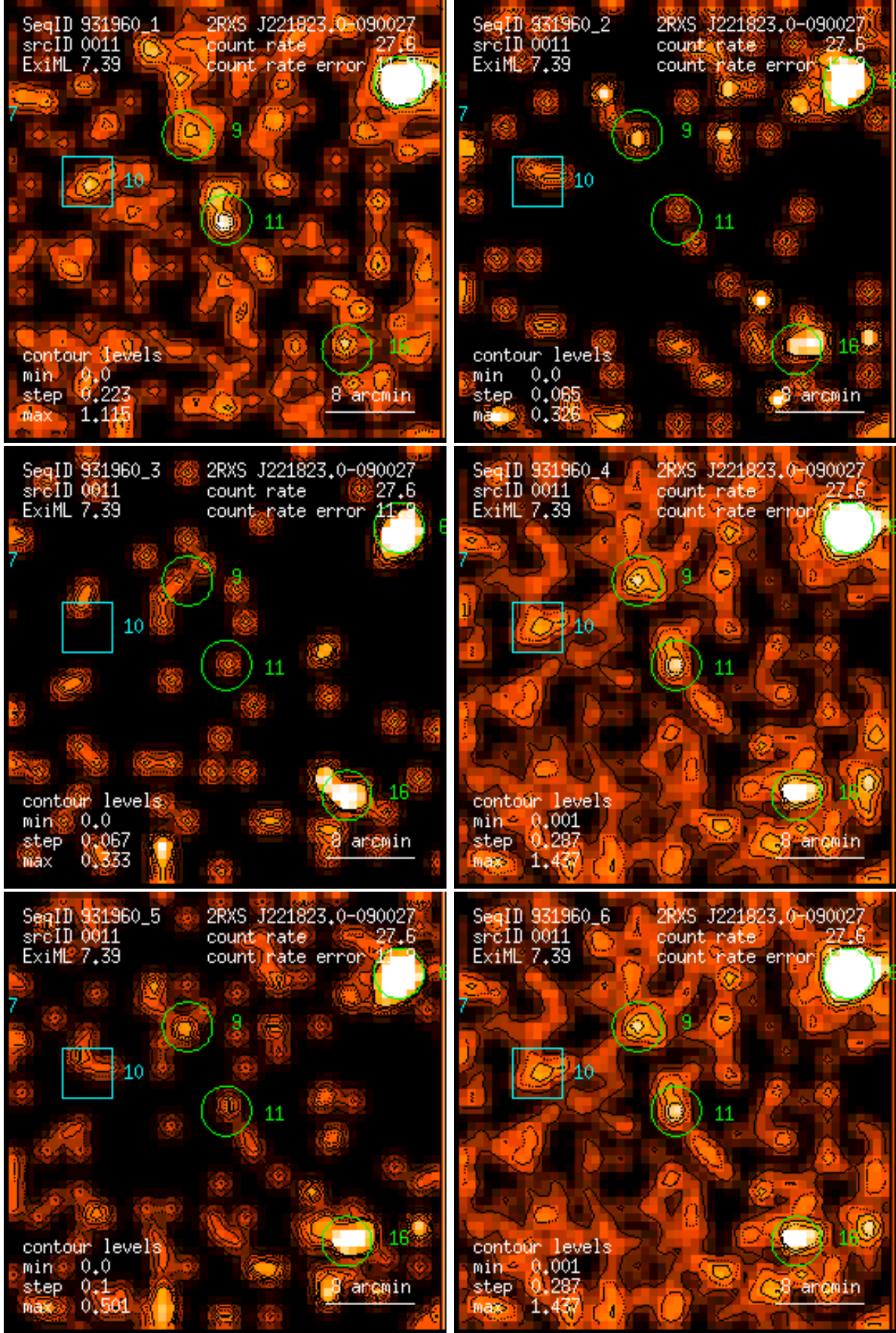
Figure 11: RASS 931960: detection 0011: band rate images, Gaussian filter: (1) PSPC channels 11 – 41, (2) 52 – 90, (3) 91 – 201, (4) 11 – 235, (5) 52 – 201, (6) 11 – 201. Broad band rates in counts/ks. Band rate contour levels in counts/ks/arcmin 2 .
