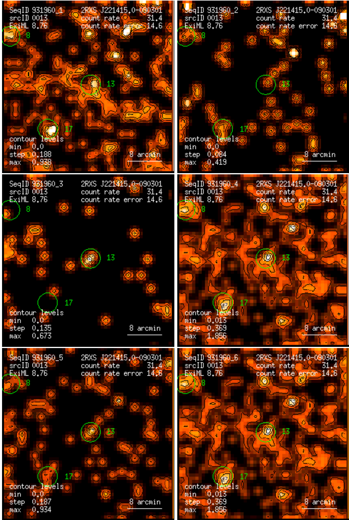
Figure 13: RASS 931960: detection 0013: band rate images, Gaussian filter: (1) PSPC channels 11 – 41, (2) 52 – 90, (3) 91 – 201, (4) 11 – 235, (5) 52 – 201, (6) 11 – 201. Broad band rates in counts/ks. Band rate contour levels in counts/ks/arcmin 2 .
