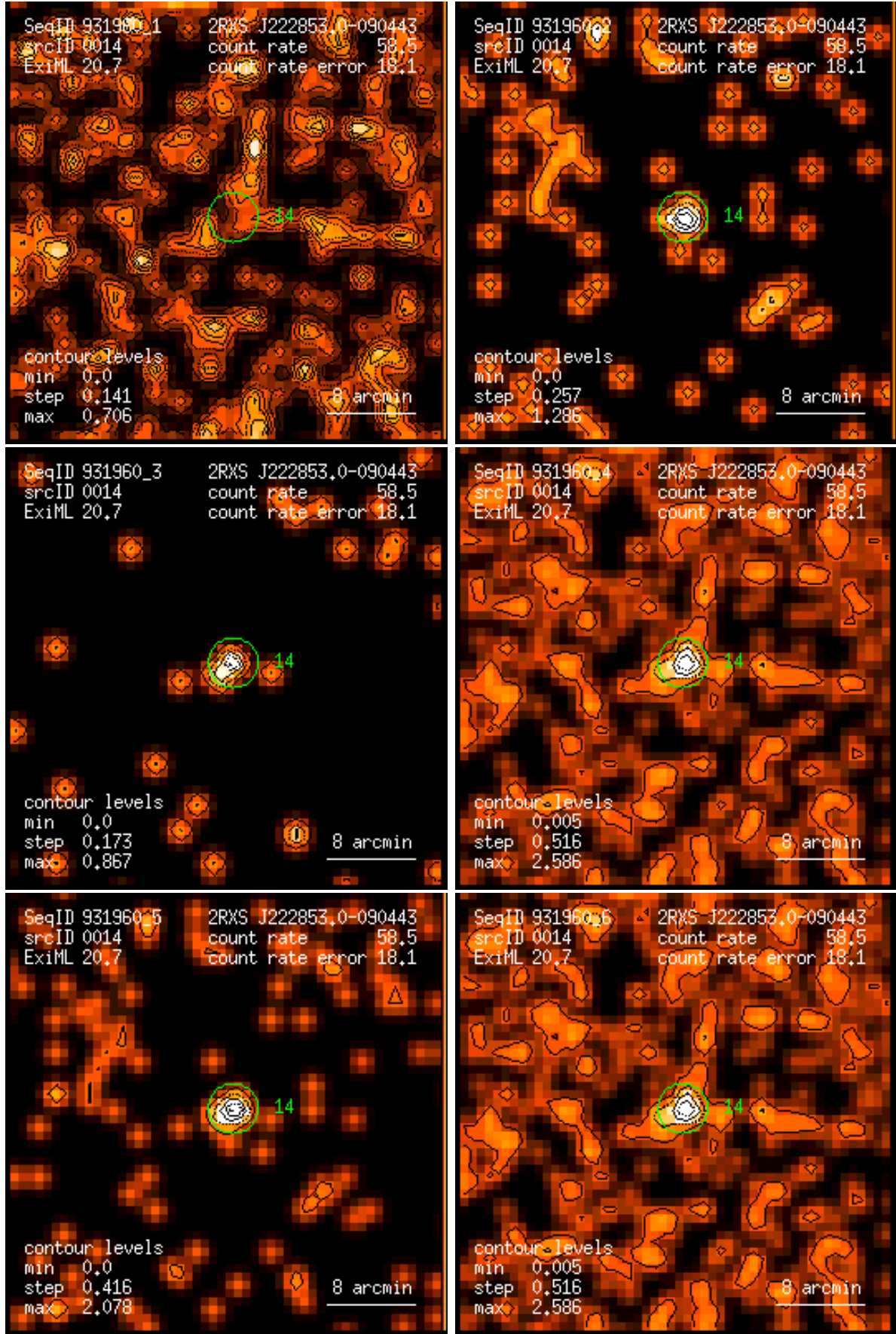
Figure 14: RASS 931960: detection 0014: band rate images, Gaussian filter: (1) PSPC channels 11 – 41, (2) 52 – 90, (3) 91 – 201, (4) 11 – 235, (5) 52 – 201, (6) 11 – 201. Broad band rates in counts/ks. Band rate contour levels in counts/ks/arcmin 2 .
