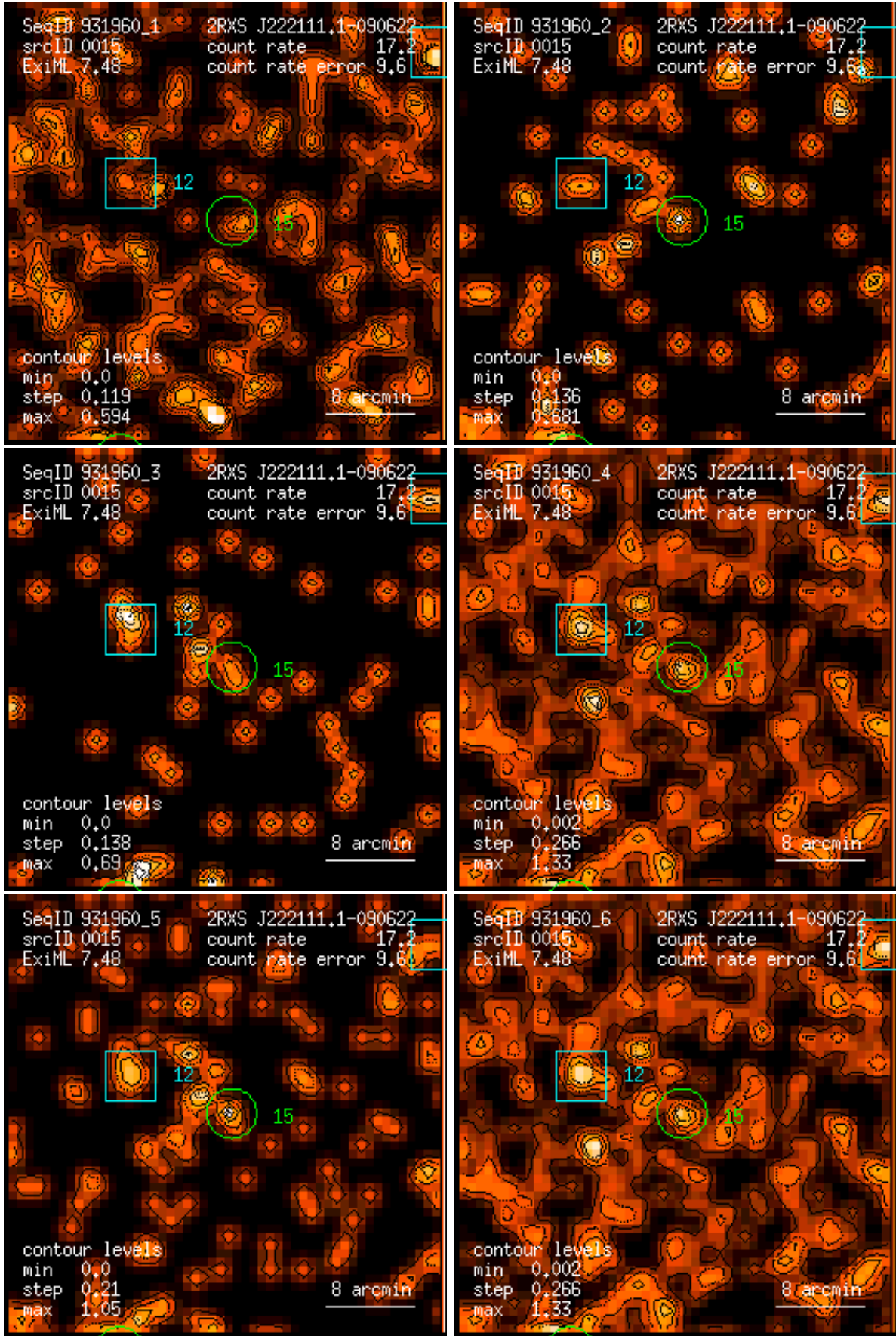
Figure 15: RASS 931960: detection 0015: band rate images, Gaussian filter: (1) PSPC channels 11 – 41, (2) 52 – 90, (3) 91 – 201, (4) 11 – 235, (5) 52 – 201, (6) 11 – 201. Broad band rates in counts/ks. Band rate contour levels in counts/ks/arcmin 2 .
