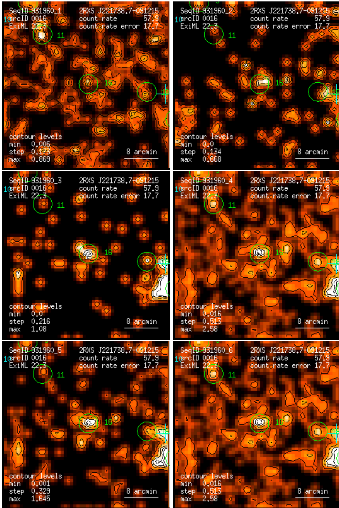
Figure 16: RASS 931960: detection 0016: band rate images, Gaussian filter: (1) PSPC channels 11 – 41, (2) 52 – 90, (3) 91 – 201, (4) 11 – 235, (5) 52 – 201, (6) 11 – 201. Broad band rates in counts/ks. Band rate contour levels in counts/ks/arcmin 2 .
