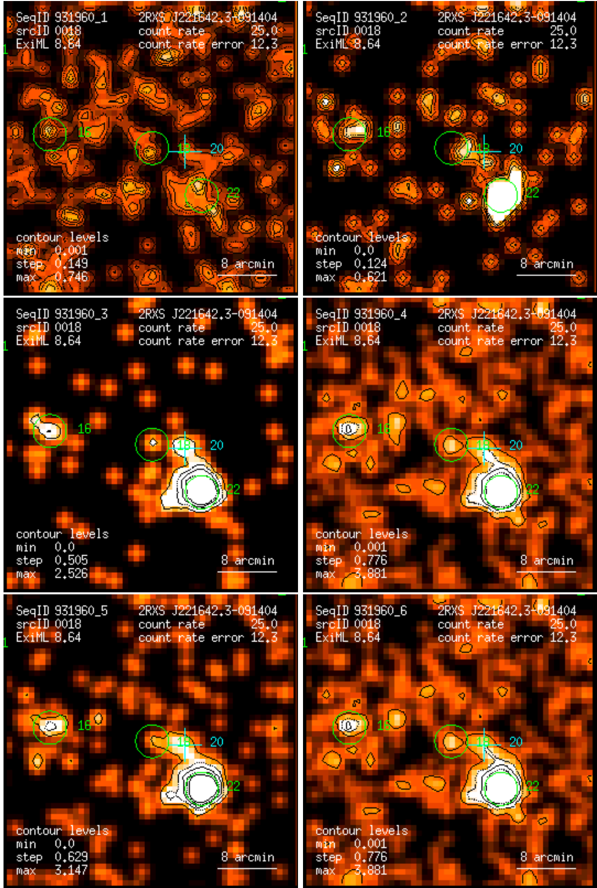
Figure 18: RASS 931960: detection 0018: band rate images, Gaussian filter: (1) PSPC channels 11 – 41, (2) 52 – 90, (3) 91 – 201, (4) 11 – 235, (5) 52 – 201, (6) 11 – 201. Broad band rates in counts/ks. Band rate contour levels in counts/ks/arcmin 2 .
