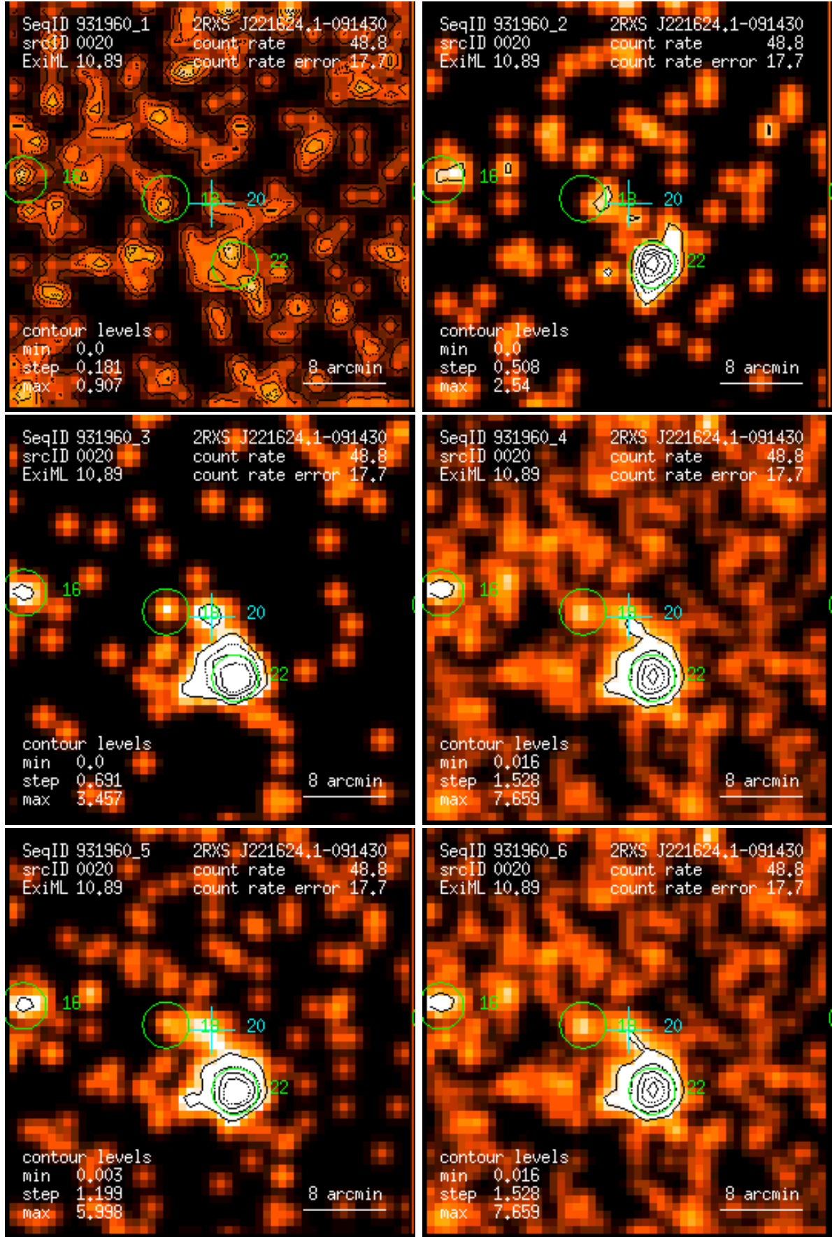
Figure 20: RASS 931960: detection 0020: band rate images, Gaussian filter: (1) PSPC channels 11 – 41, (2) 52 – 90, (3) 91 – 201, (4) 11 – 235, (5) 52 – 201, (6) 11 – 201. Broad band rates in counts/ks. Band rate contour levels in counts/ks/arcmin 2 .
