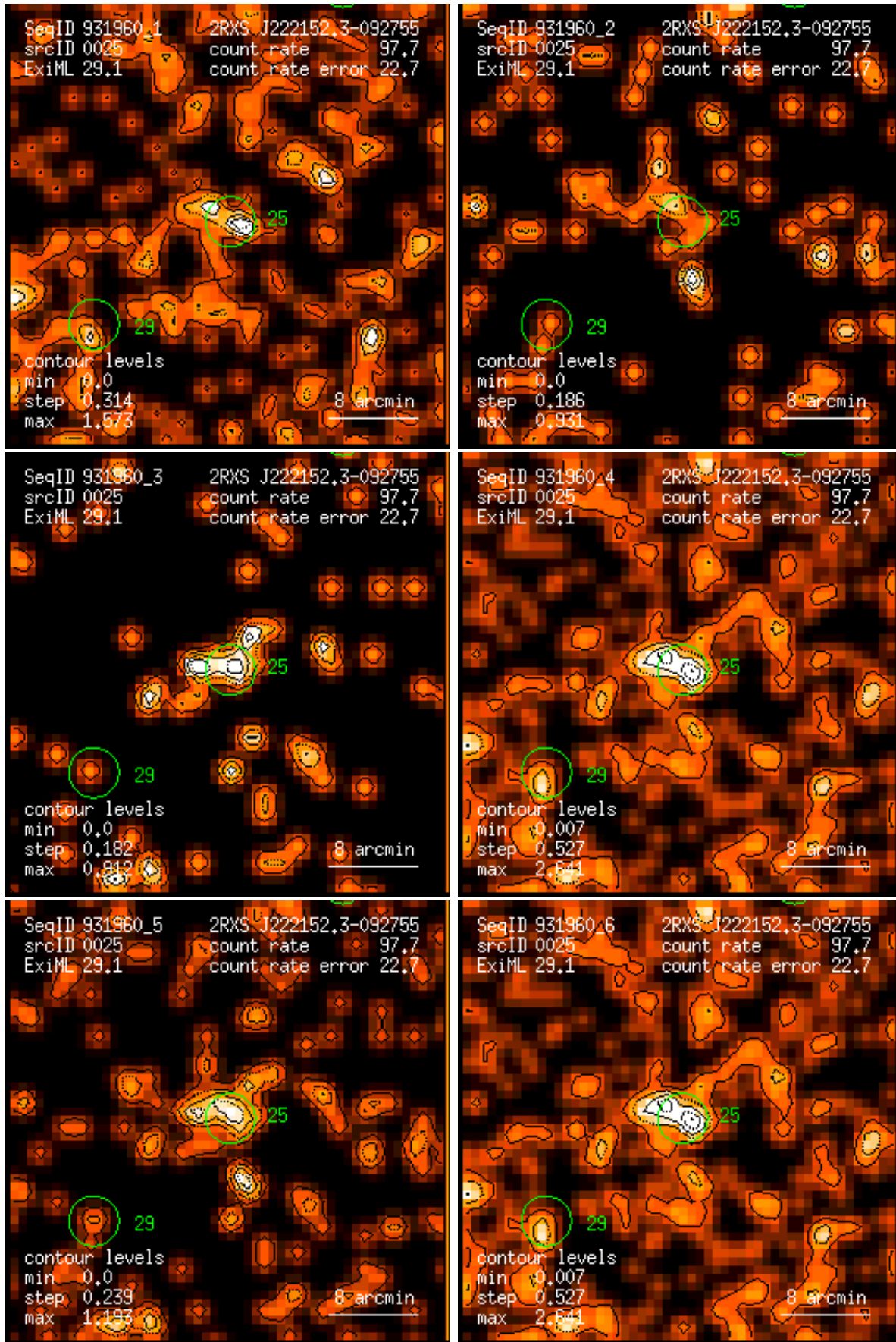
Figure 25: RASS 931960: detection 0025: band rate images, Gaussian filter: (1) PSPC channels 11 – 41, (2) 52 – 90, (3) 91 – 201, (4) 11 – 235, (5) 52 – 201, (6) 11 – 201. Broad band rates in counts/ks. Band rate contour levels in counts/ks/arcmin 2 .
