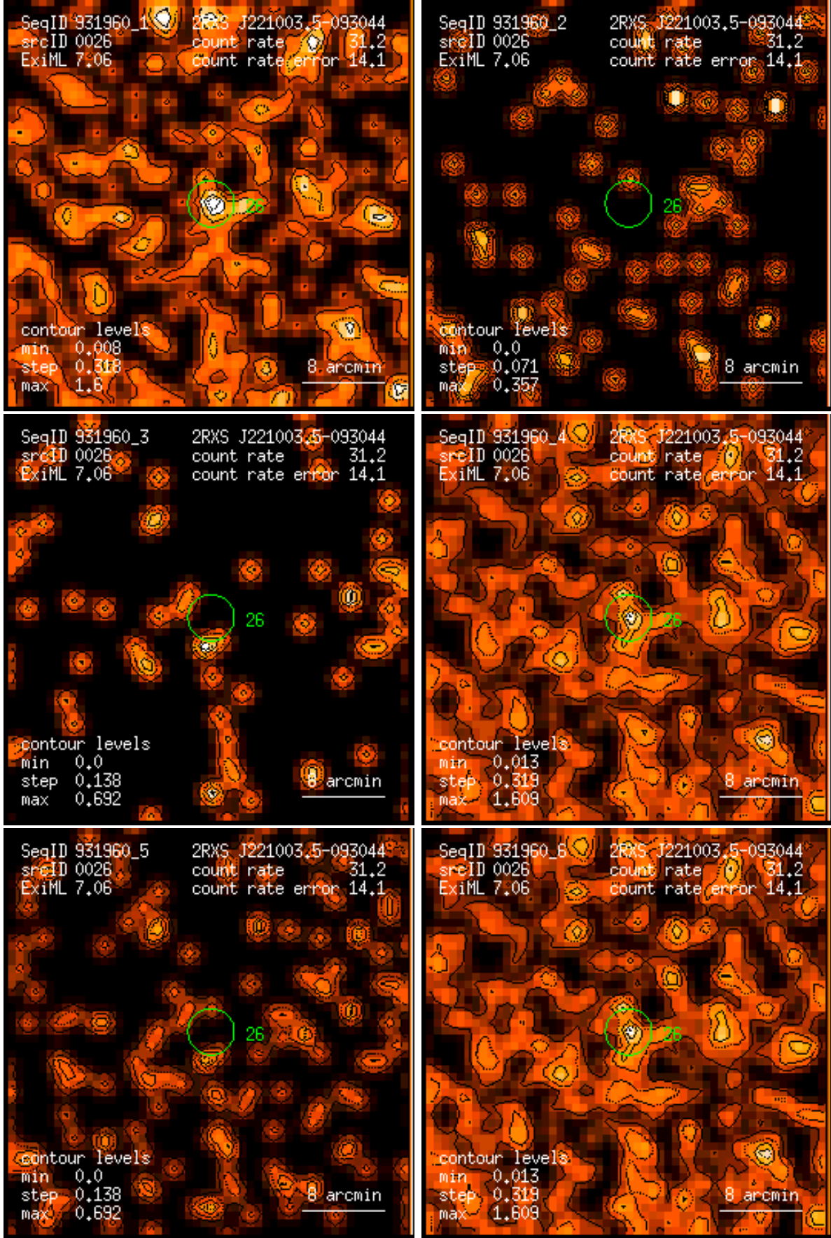
Figure 26: RASS 931960: detection 0026: band rate images, Gaussian filter: (1) PSPC channels 11 – 41, (2) 52 – 90, (3) 91 – 201, (4) 11 – 235, (5) 52 – 201, (6) 11 – 201. Broad band rates in counts/ks. Band rate contour levels in counts/ks/arcmin 2 .
