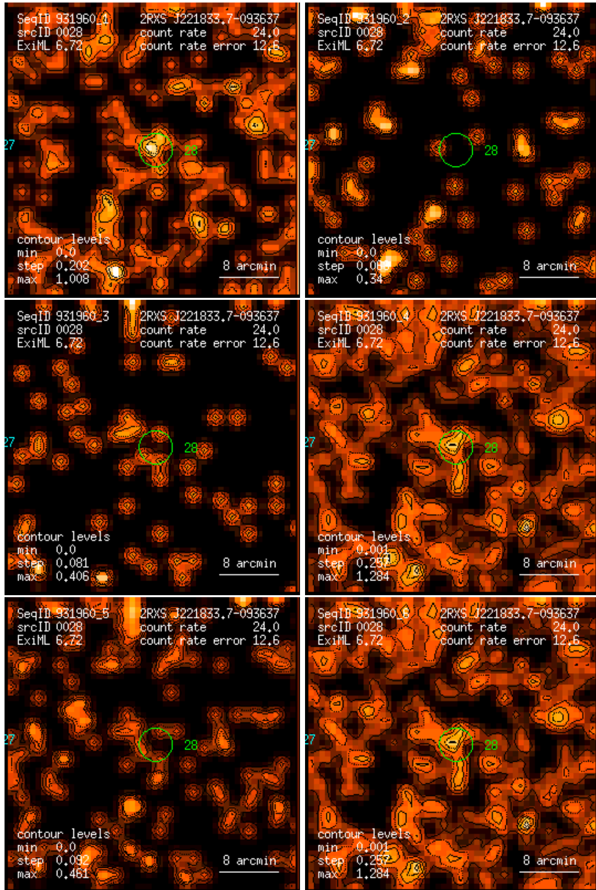
Figure 28: RASS 931960: detection 0028: band rate images, Gaussian filter: (1) PSPC channels 11 – 41, (2) 52 – 90, (3) 91 – 201, (4) 11 – 235, (5) 52 – 201, (6) 11 – 201. Broad band rates in counts/ks. Band rate contour levels in counts/ks/arcmin 2 .
