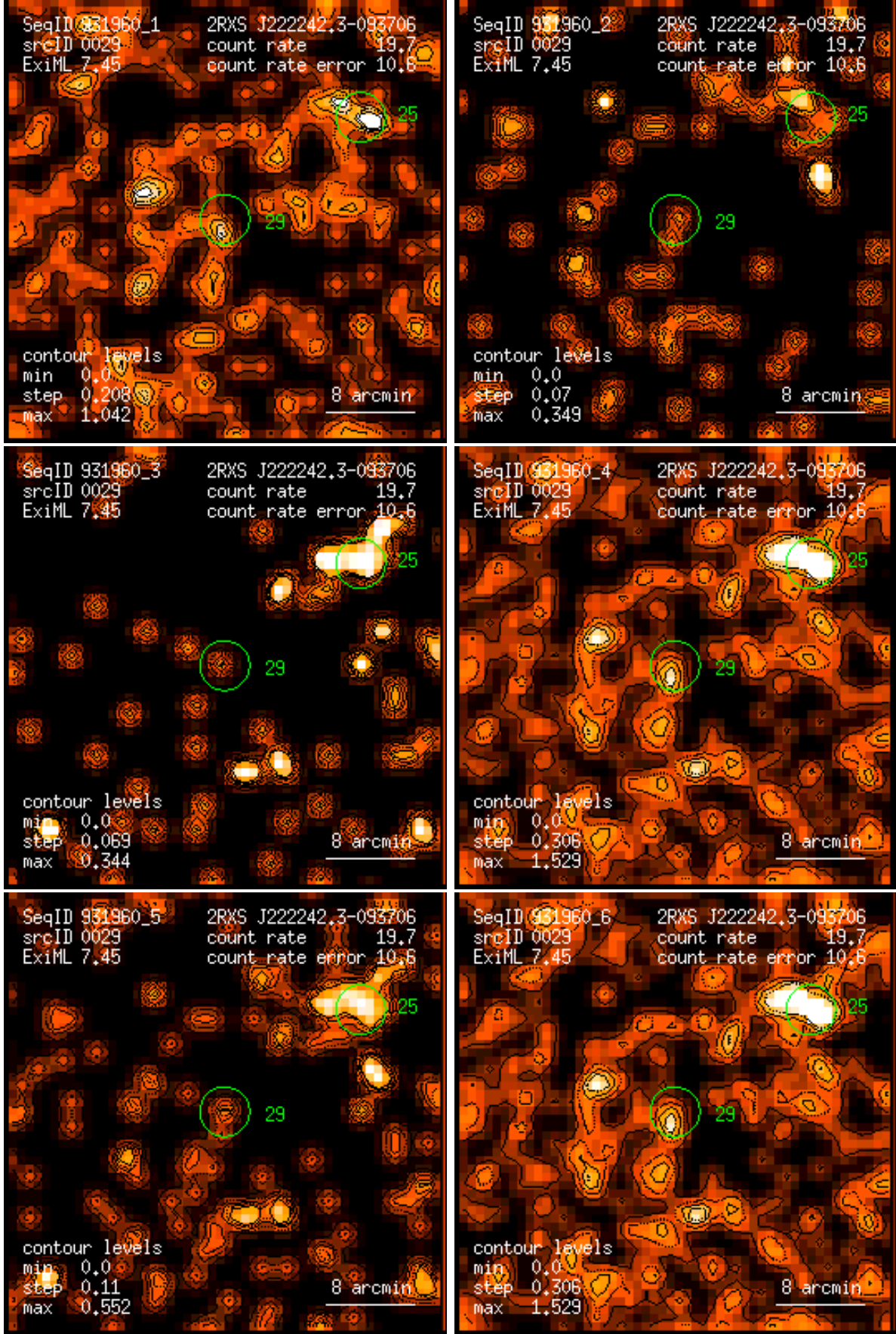
Figure 29: RASS 931960: detection 0029: band rate images, Gaussian filter: (1) PSPC channels 11 – 41, (2) 52 – 90, (3) 91 – 201, (4) 11 – 235, (5) 52 – 201, (6) 11 – 201. Broad band rates in counts/ks. Band rate contour levels in counts/ks/arcmin 2 .
