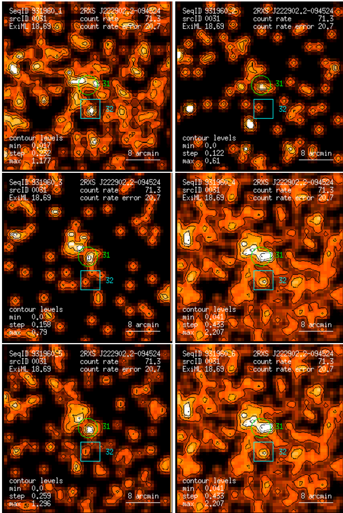
Figure 31: RASS 931960: detection 0031: band rate images, Gaussian filter: (1) PSPC channels 11 – 41, (2) 52 – 90, (3) 91 – 201, (4) 11 – 235, (5) 52 – 201, (6) 11 – 201. Broad band rates in counts/ks. Band rate contour levels in counts/ks/arcmin 2 .
