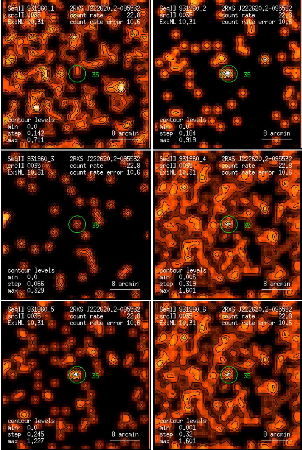
Figure 35: RASS 931960: detection 0035: band rate images, Gaussian filter: (1) PSPC channels 11 – 41, (2) 52 – 90, (3) 91 – 201, (4) 11 – 235, (5) 52 – 201, (6) 11 – 201. Broad band rates in counts/ks. Band rate contour levels in counts/ks/arcmin 2 .
