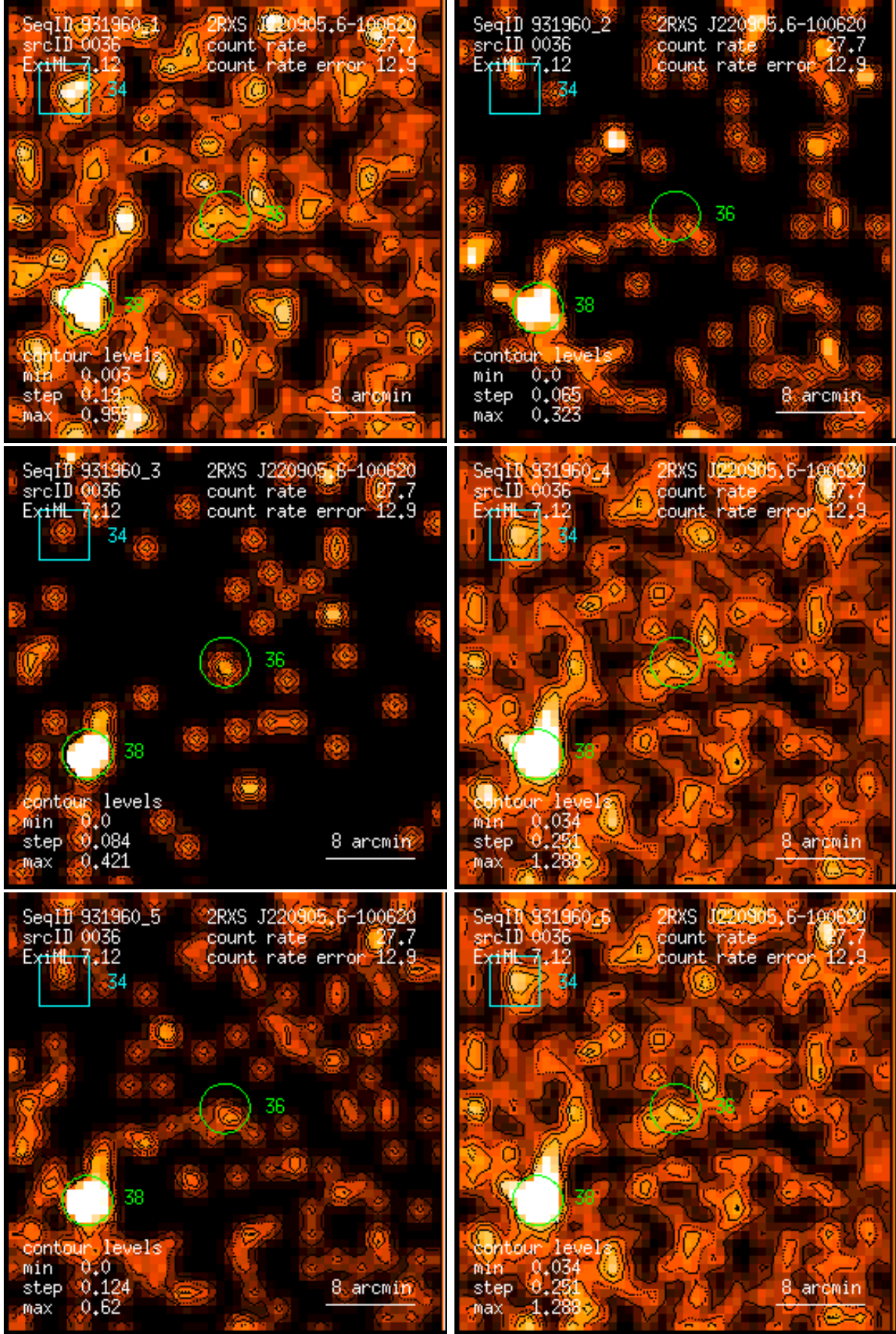
Figure 36: RASS 931960: detection 0036: band rate images, Gaussian filter: (1) PSPC channels 11 – 41, (2) 52 – 90, (3) 91 – 201, (4) 11 – 235, (5) 52 – 201, (6) 11 – 201. Broad band rates in counts/ks. Band rate contour levels in counts/ks/arcmin 2 .
