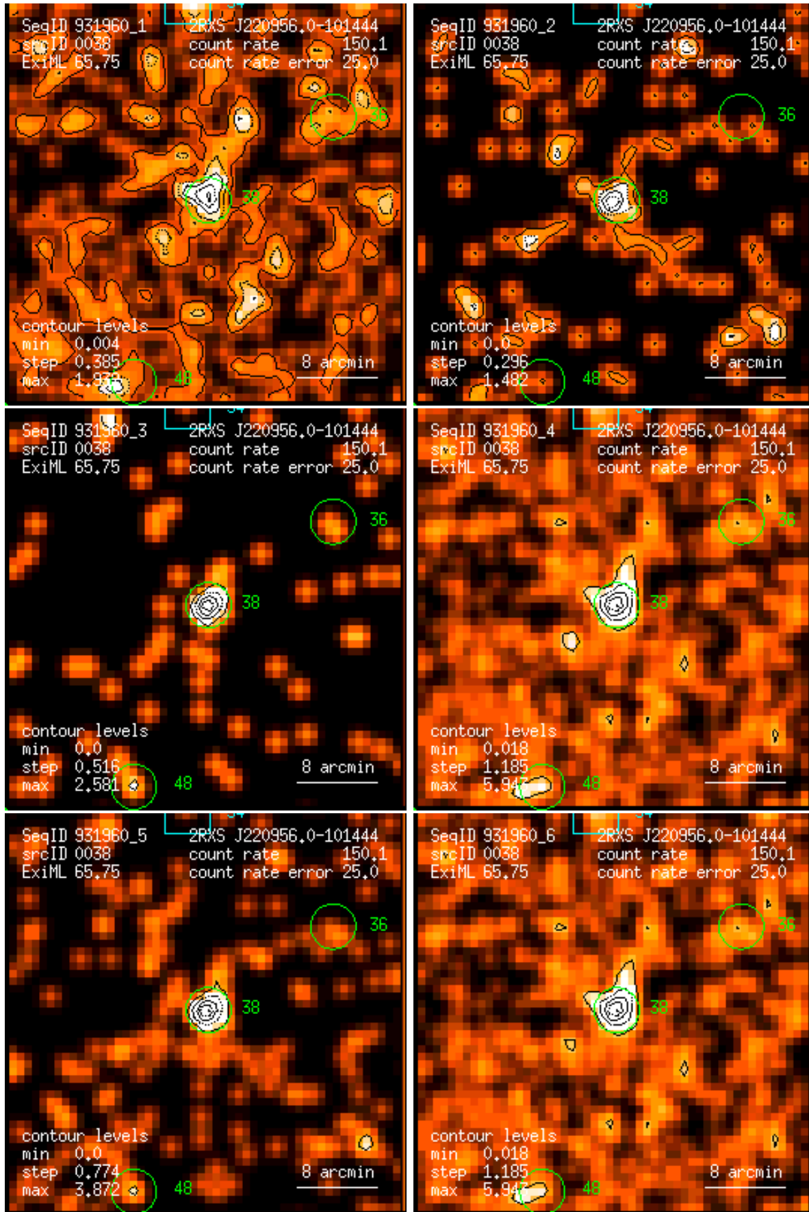
Figure 38: RASS 931960: detection 0038: band rate images, Gaussian filter: (1) PSPC channels 11 – 41, (2) 52 – 90, (3) 91 – 201, (4) 11 – 235, (5) 52 – 201, (6) 11 – 201. Broad band rates in counts/ks. Band rate contour levels in counts/ks/arcmin 2 .
