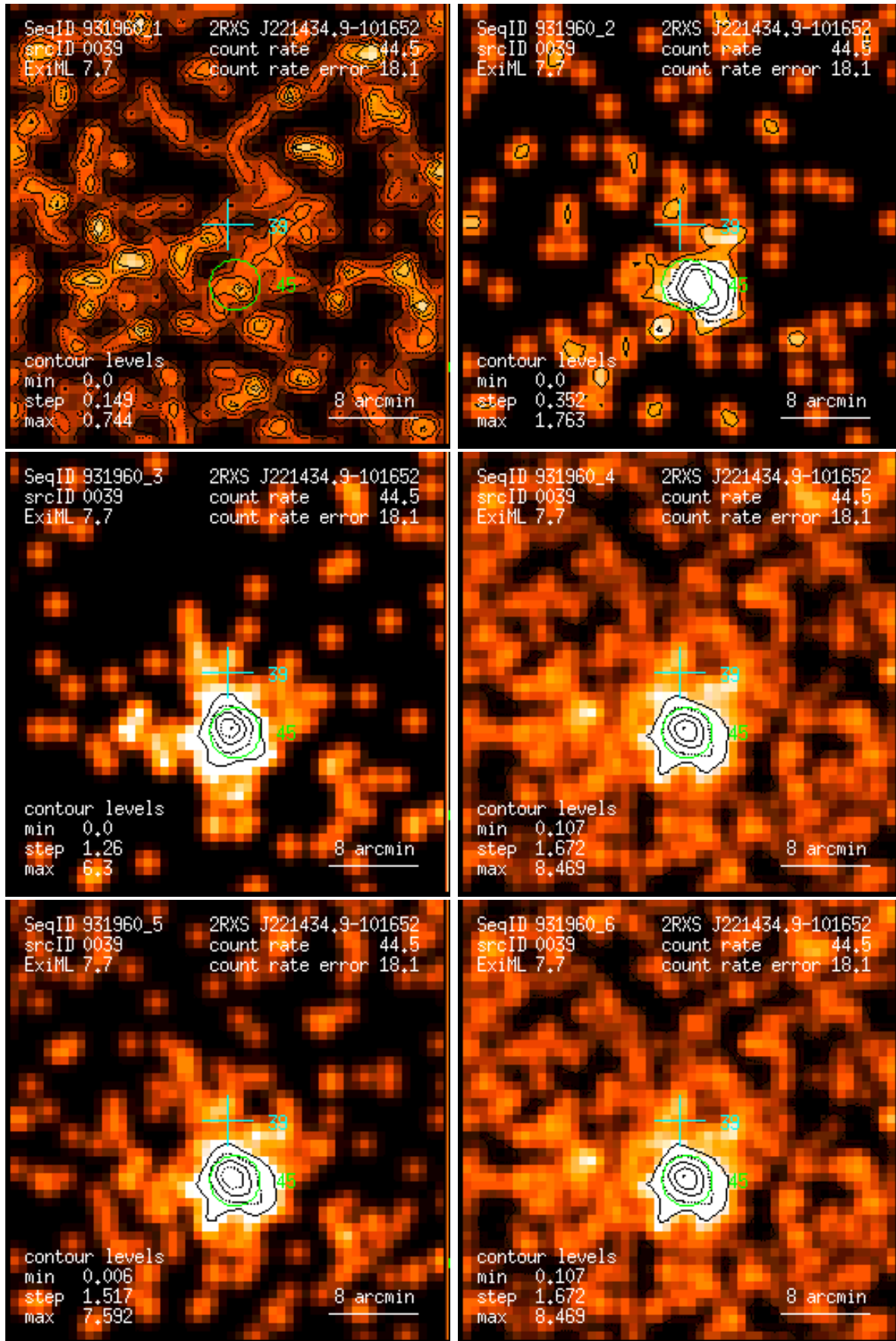
Figure 39: RASS 931960: detection 0039: band rate images, Gaussian filter: (1) PSPC channels 11 – 41, (2) 52 – 90, (3) 91 – 201, (4) 11 – 235, (5) 52 – 201, (6) 11 – 201. Broad band rates in counts/ks. Band rate contour levels in counts/ks/arcmin 2 .
