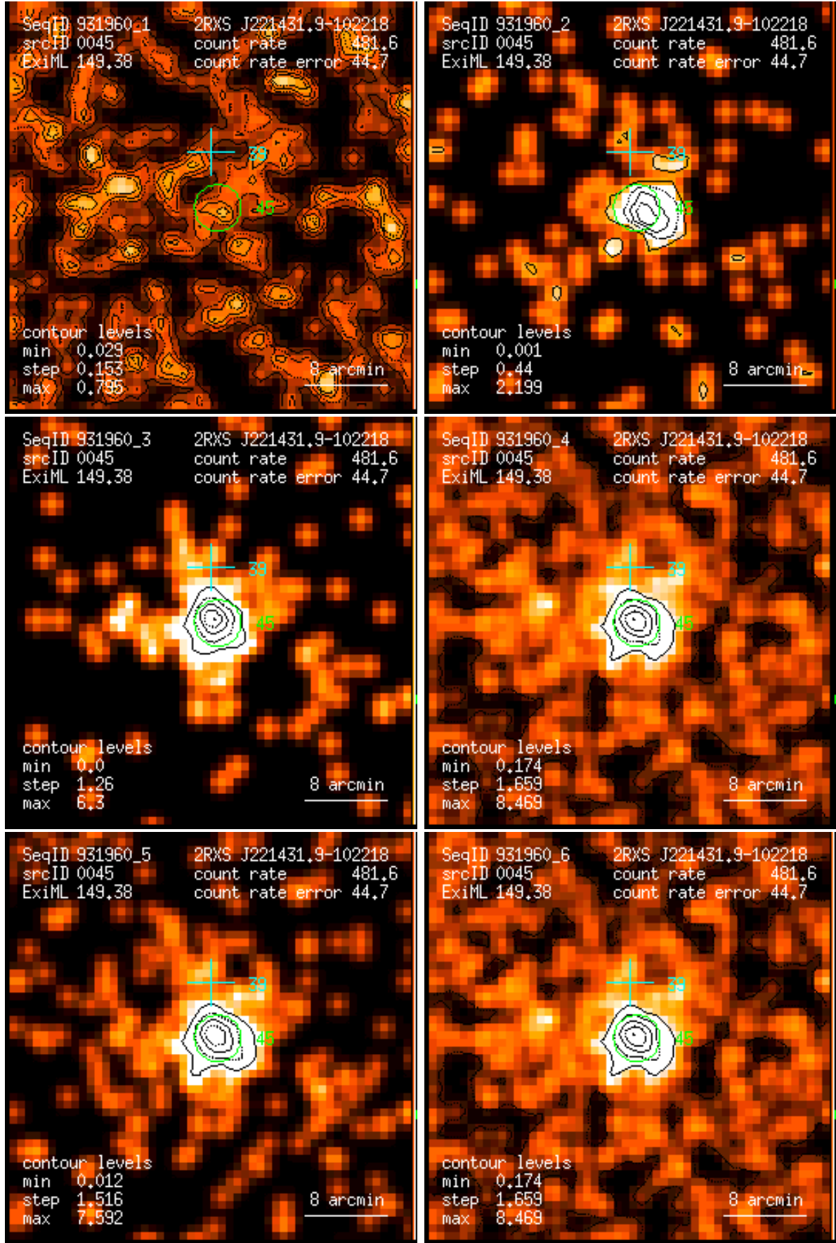
Figure 45: RASS 931960: detection 0045: band rate images, Gaussian filter: (1) PSPC channels 11 – 41, (2) 52 – 90, (3) 91 – 201, (4) 11 – 235, (5) 52 – 201, (6) 11 – 201. Broad band rates in counts/ks. Band rate contour levels in counts/ks/arcmin 2 .
