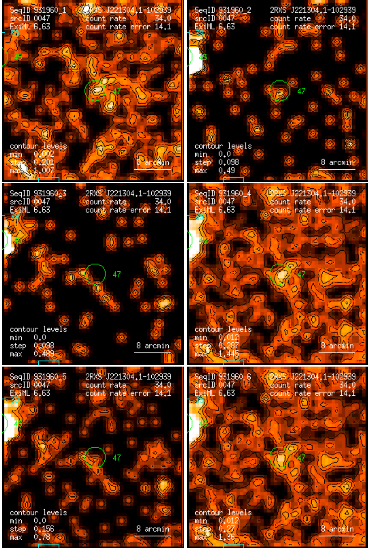
Figure 47: RASS 931960: detection 0047: band rate images, Gaussian filter: (1) PSPC channels 11 – 41, (2) 52 – 90, (3) 91 – 201, (4) 11 – 235, (5) 52 – 201, (6) 11 – 201. Broad band rates in counts/ks. Band rate contour levels in counts/ks/arcmin 2 .
