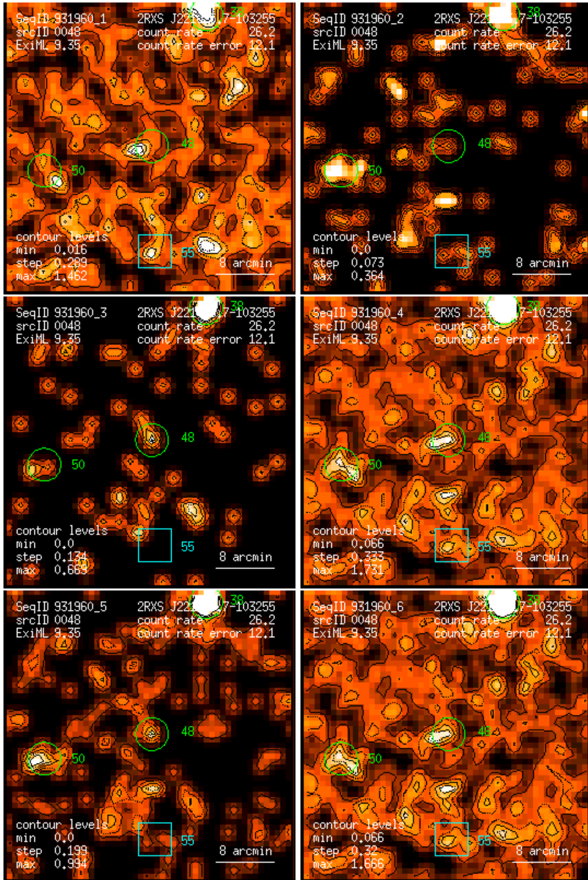
Figure 48: RASS 931960: detection 0048: band rate images, Gaussian filter: (1) PSPC channels 11 – 41, (2) 52 – 90, (3) 91 – 201, (4) 11 – 235, (5) 52 – 201, (6) 11 – 201. Broad band rates in counts/ks. Band rate contour levels in counts/ks/arcmin 2 .
