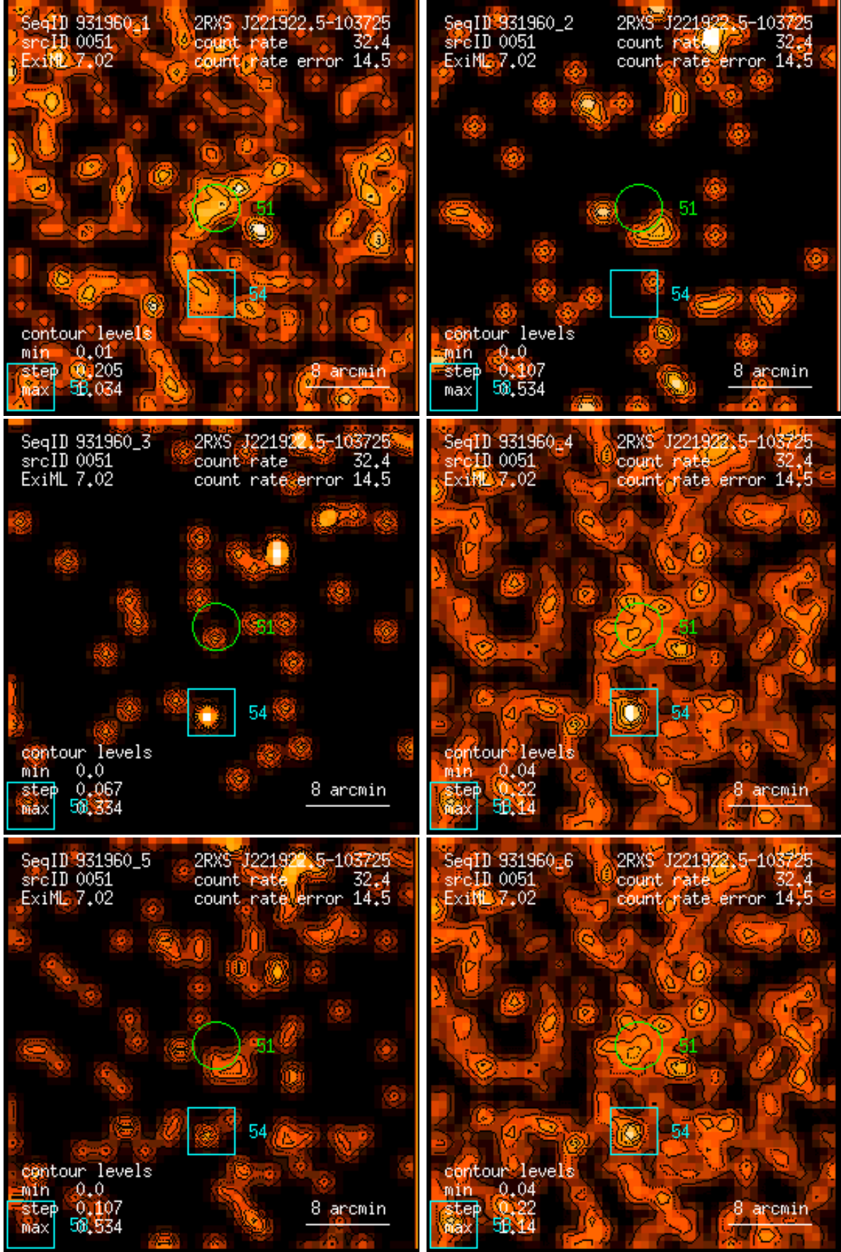
Figure 51: RASS 931960: detection 0051: band rate images, Gaussian filter: (1) PSPC channels 11 – 41, (2) 52 – 90, (3) 91 – 201, (4) 11 – 235, (5) 52 – 201, (6) 11 – 201. Broad band rates in counts/ks. Band rate contour levels in counts/ks/arcmin 2 .
