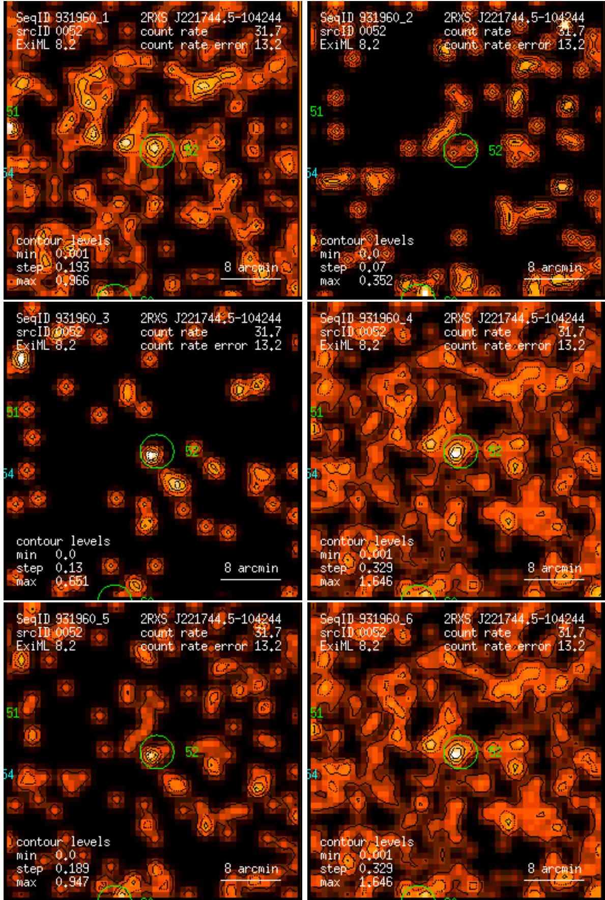
Figure 52: RASS 931960: detection 0052: band rate images, Gaussian filter: (1) PSPC channels 11 – 41, (2) 52 – 90, (3) 91 – 201, (4) 11 – 235, (5) 52 – 201, (6) 11 – 201. Broad band rates in counts/ks. Band rate contour levels in counts/ks/arcmin 2 .
