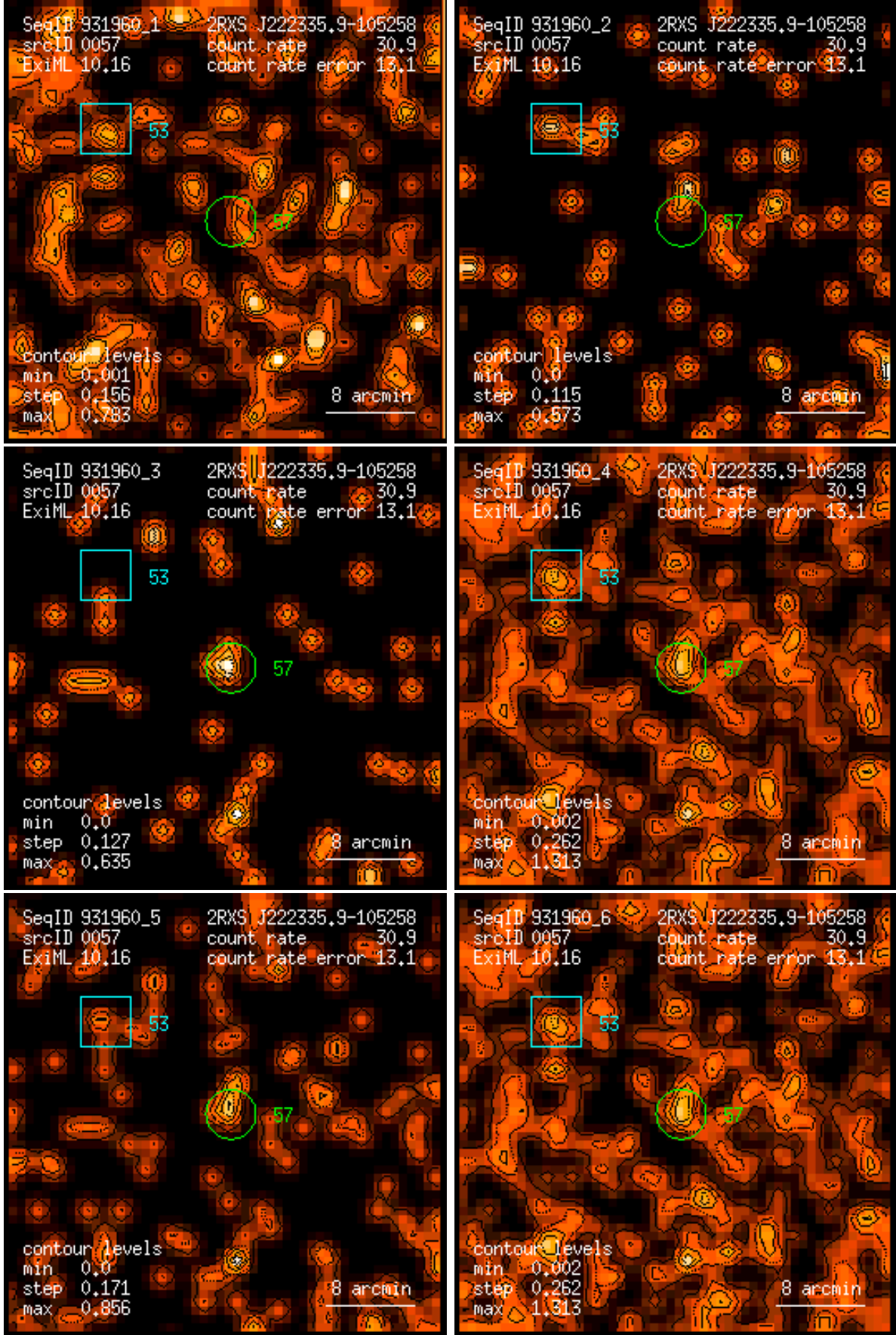
Figure 57: RASS 931960: detection 0057: band rate images, Gaussian filter: (1) PSPC channels 11 – 41, (2) 52 – 90, (3) 91 – 201, (4) 11 – 235, (5) 52 – 201, (6) 11 – 201. Broad band rates in counts/ks. Band rate contour levels in counts/ks/arcmin 2 .
