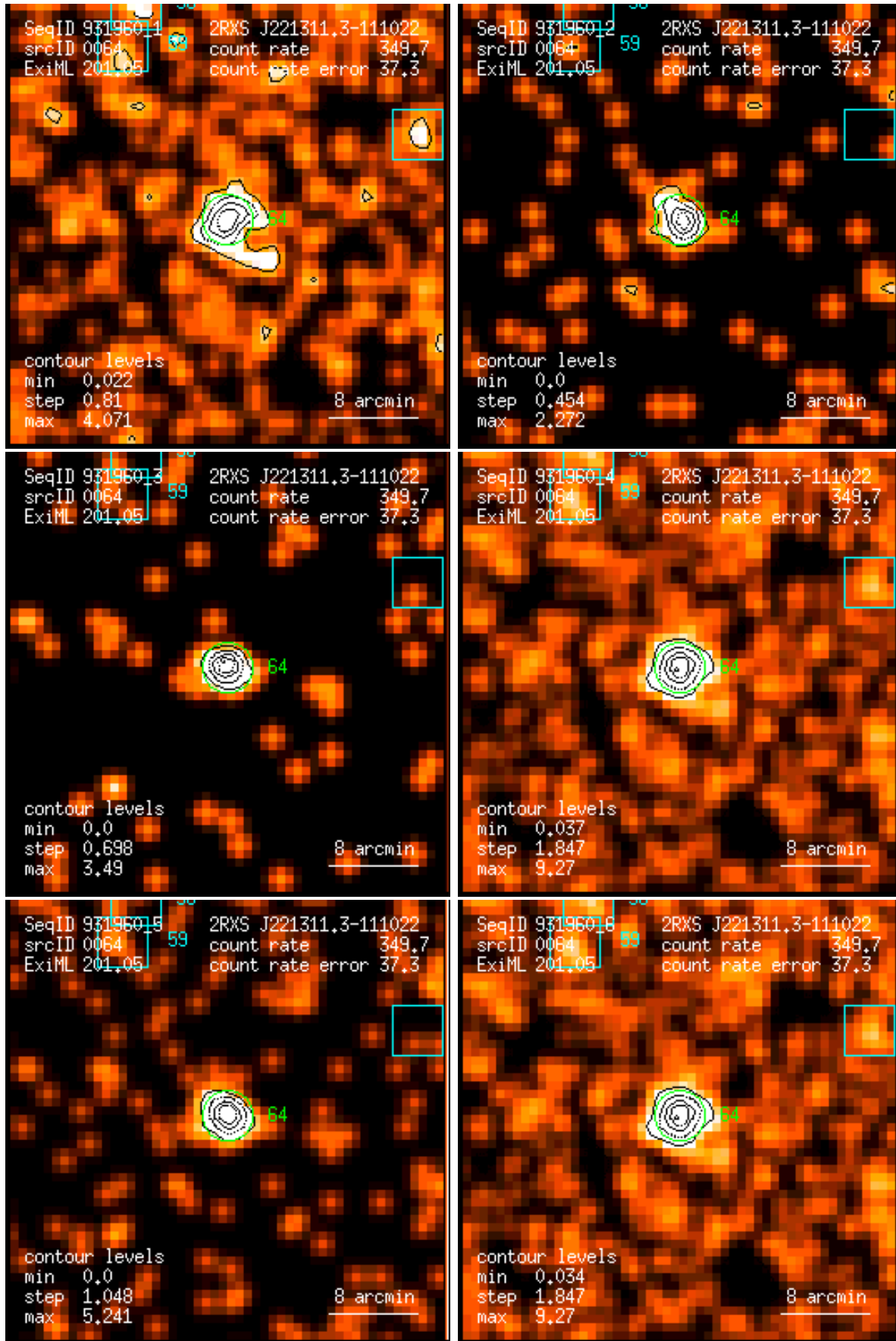
Figure 64: RASS 931960: detection 0064: band rate images, Gaussian filter: (1) PSPC channels 11 – 41, (2) 52 – 90, (3) 91 – 201, (4) 11 – 235, (5) 52 – 201, (6) 11 – 201. Broad band rates in counts/ks. Band rate contour levels in counts/ks/arcmin 2 .
