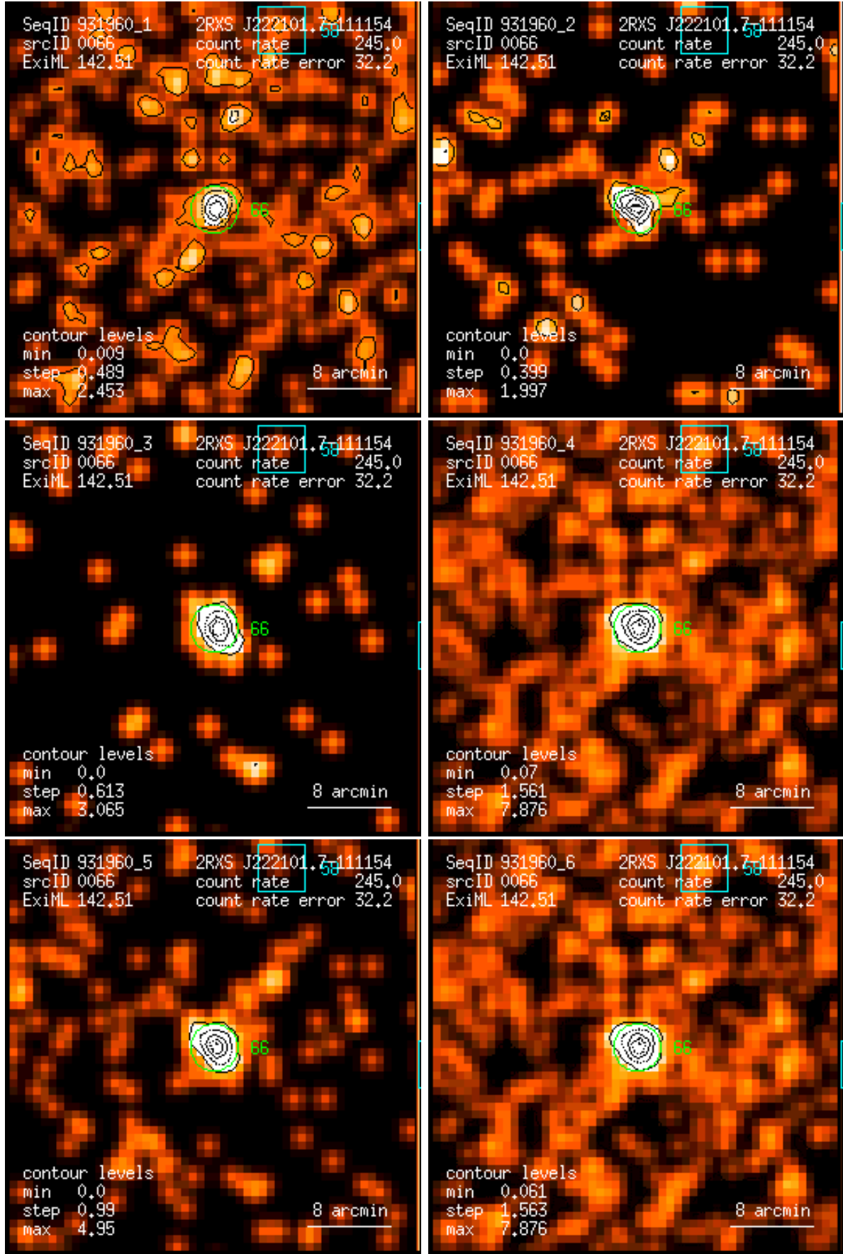
Figure 66: RASS 931960: detection 0066: band rate images, Gaussian filter: (1) PSPC channels 11 – 41, (2) 52 – 90, (3) 91 – 201, (4) 11 – 235, (5) 52 – 201, (6) 11 – 201. Broad band rates in counts/ks. Band rate contour levels in counts/ks/arcmin 2 .
