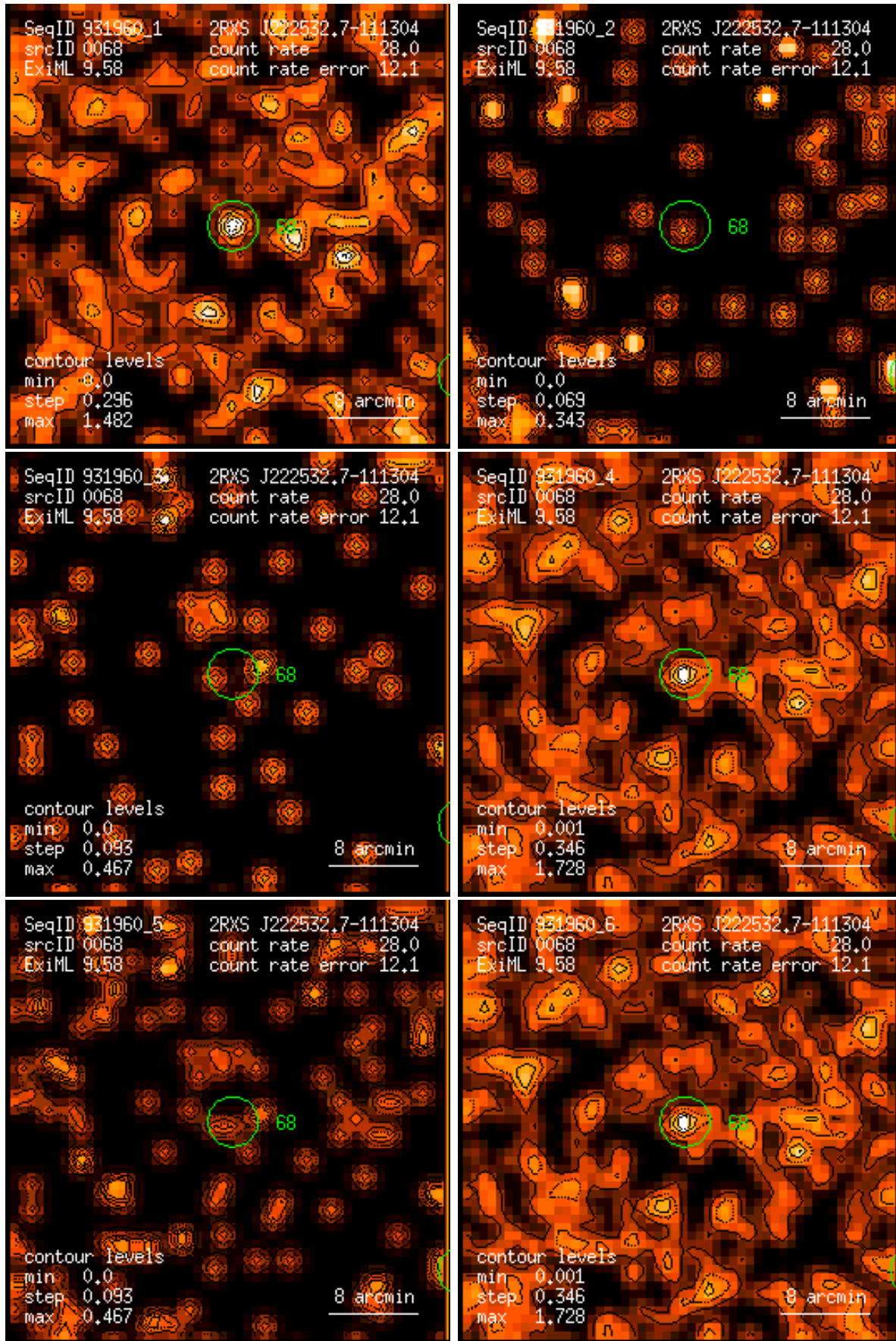
Figure 68: RASS 931960: detection 0068: band rate images, Gaussian filter: (1) PSPC channels 11 – 41, (2) 52 – 90, (3) 91 – 201, (4) 11 – 235, (5) 52 – 201, (6) 11 – 201. Broad band rates in counts/ks. Band rate contour levels in counts/ks/arcmin 2 .
