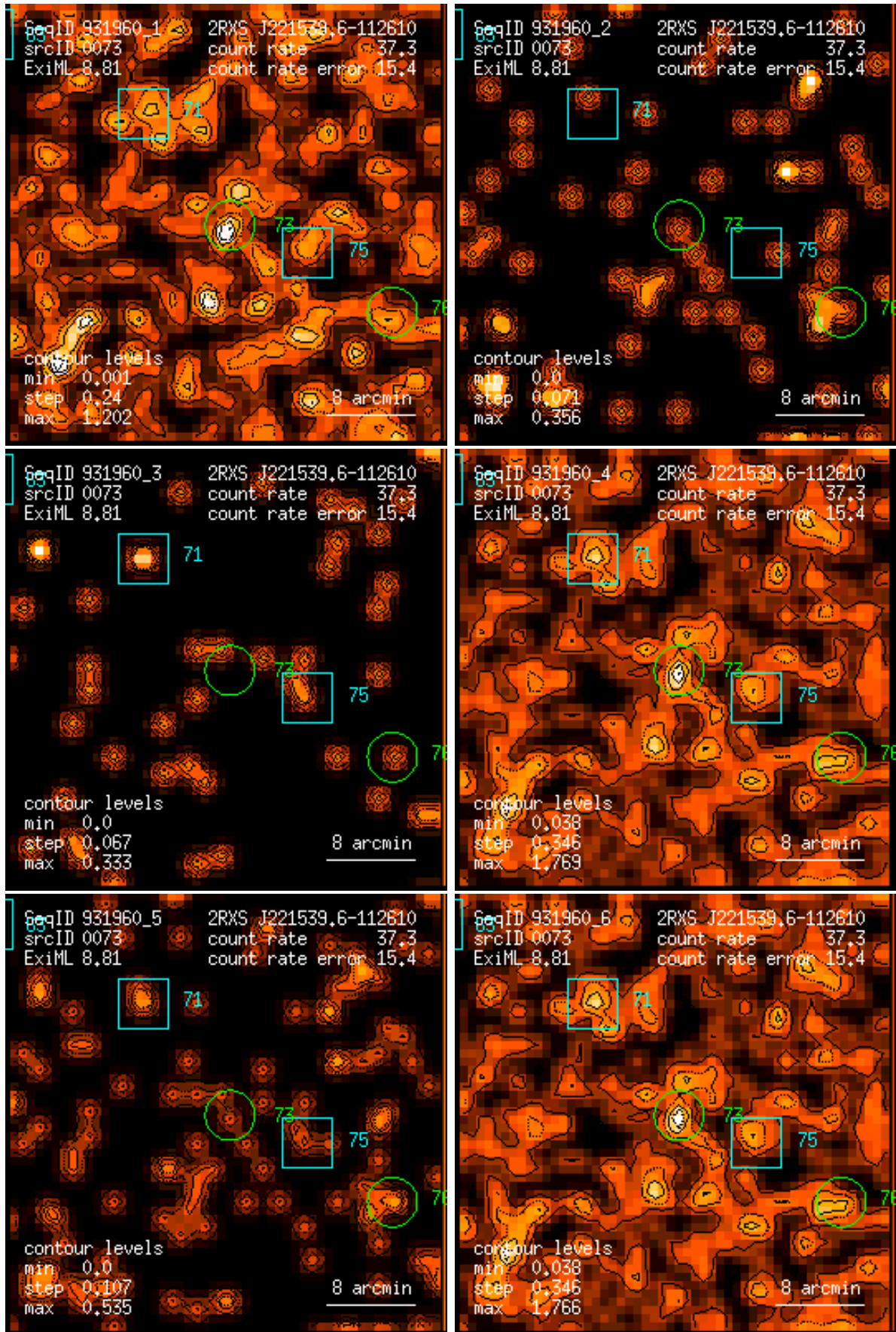
Figure 73: RASS 931960: detection 0073: band rate images, Gaussian filter: (1) PSPC channels 11 – 41, (2) 52 – 90, (3) 91 – 201, (4) 11 – 235, (5) 52 – 201, (6) 11 – 201. Broad band rates in counts/ks. Band rate contour levels in counts/ks/arcmin 2 .
