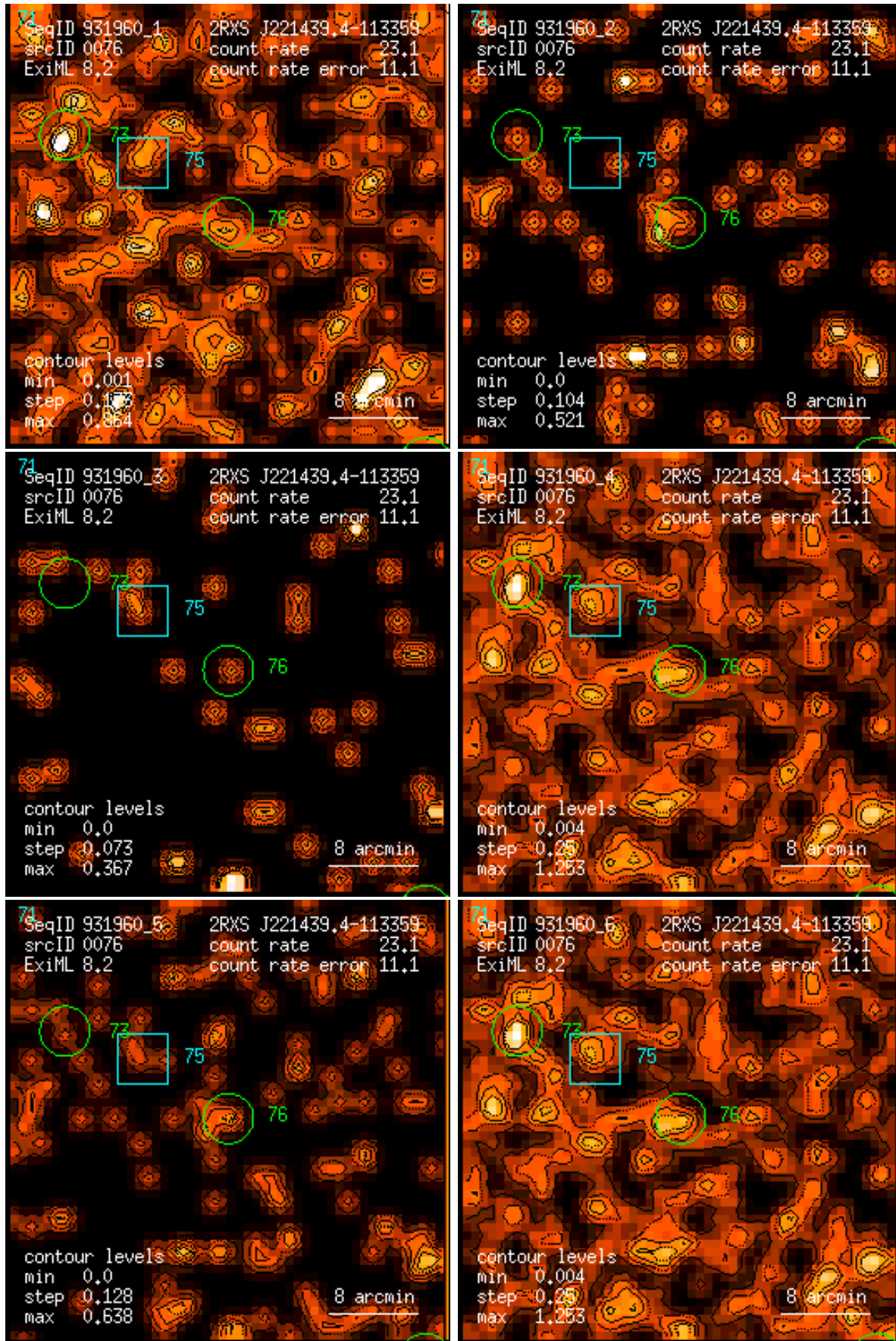
Figure 76: RASS 931960: detection 0076: band rate images, Gaussian filter: (1) PSPC channels 11 – 41, (2) 52 – 90, (3) 91 – 201, (4) 11 – 235, (5) 52 – 201, (6) 11 – 201. Broad band rates in counts/ks. Band rate contour levels in counts/ks/arcmin 2 .
