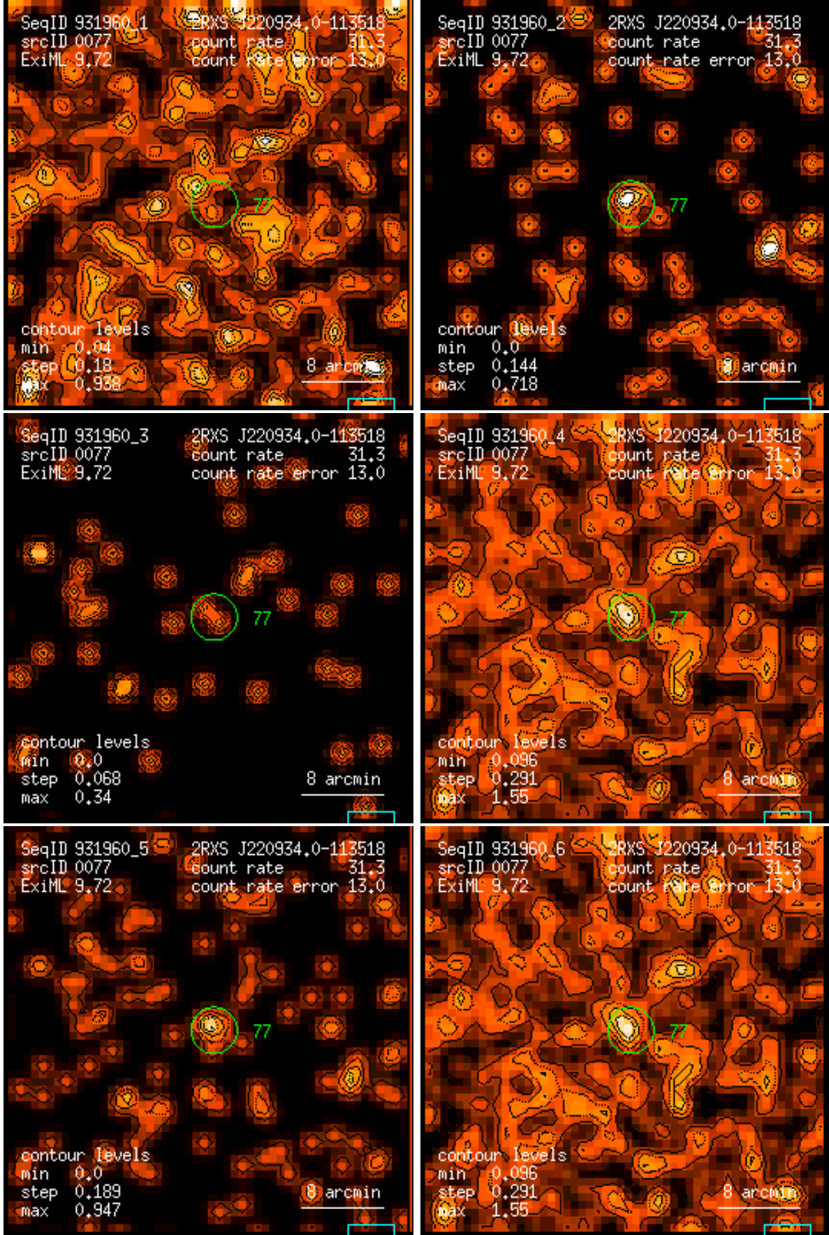
Figure 77: RASS 931960: detection 0077: band rate images, Gaussian filter: (1) PSPC channels 11 – 41, (2) 52 – 90, (3) 91 – 201, (4) 11 – 235, (5) 52 – 201, (6) 11 – 201. Broad band rates in counts/ks. Band rate contour levels in counts/ks/arcmin 2 .
