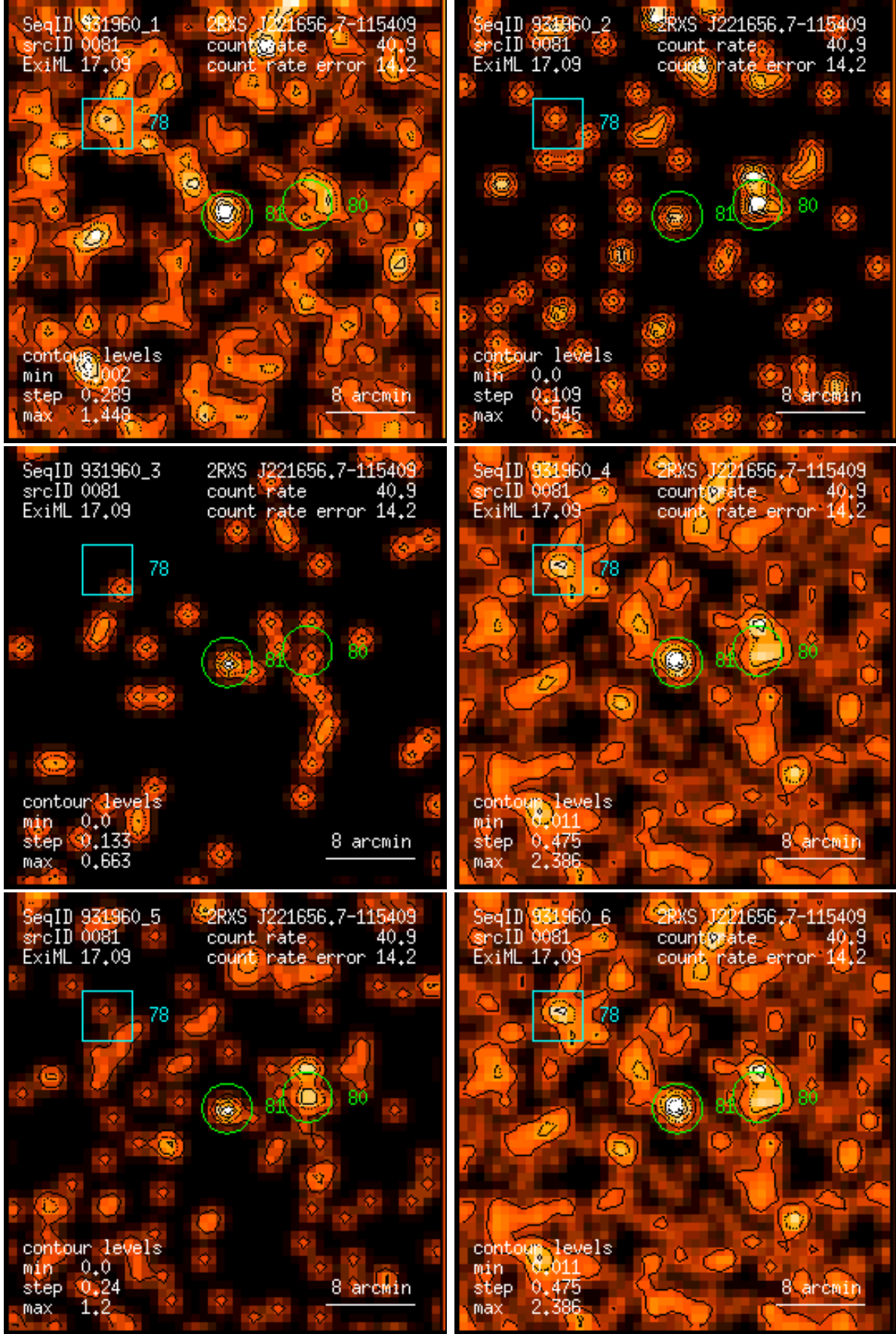
Figure 81: RASS 931960: detection 0081: band rate images, Gaussian filter: (1) PSPC channels 11 – 41, (2) 52 – 90, (3) 91 – 201, (4) 11 – 235, (5) 52 – 201, (6) 11 – 201. Broad band rates in counts/ks. Band rate contour levels in counts/ks/arcmin 2 .
