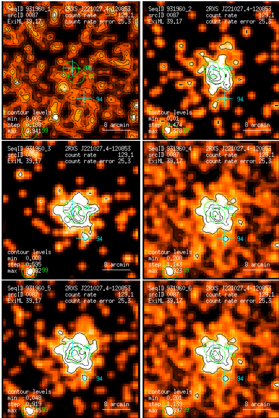
Figure 87: RASS 931960: detection 0087: band rate images, Gaussian filter: (1) PSPC channels 11 – 41, (2) 52 – 90, (3) 91 – 201, (4) 11 – 235, (5) 52 – 201, (6) 11 – 201. Broad band rates in counts/ks. Band rate contour levels in counts/ks/arcmin 2 .
