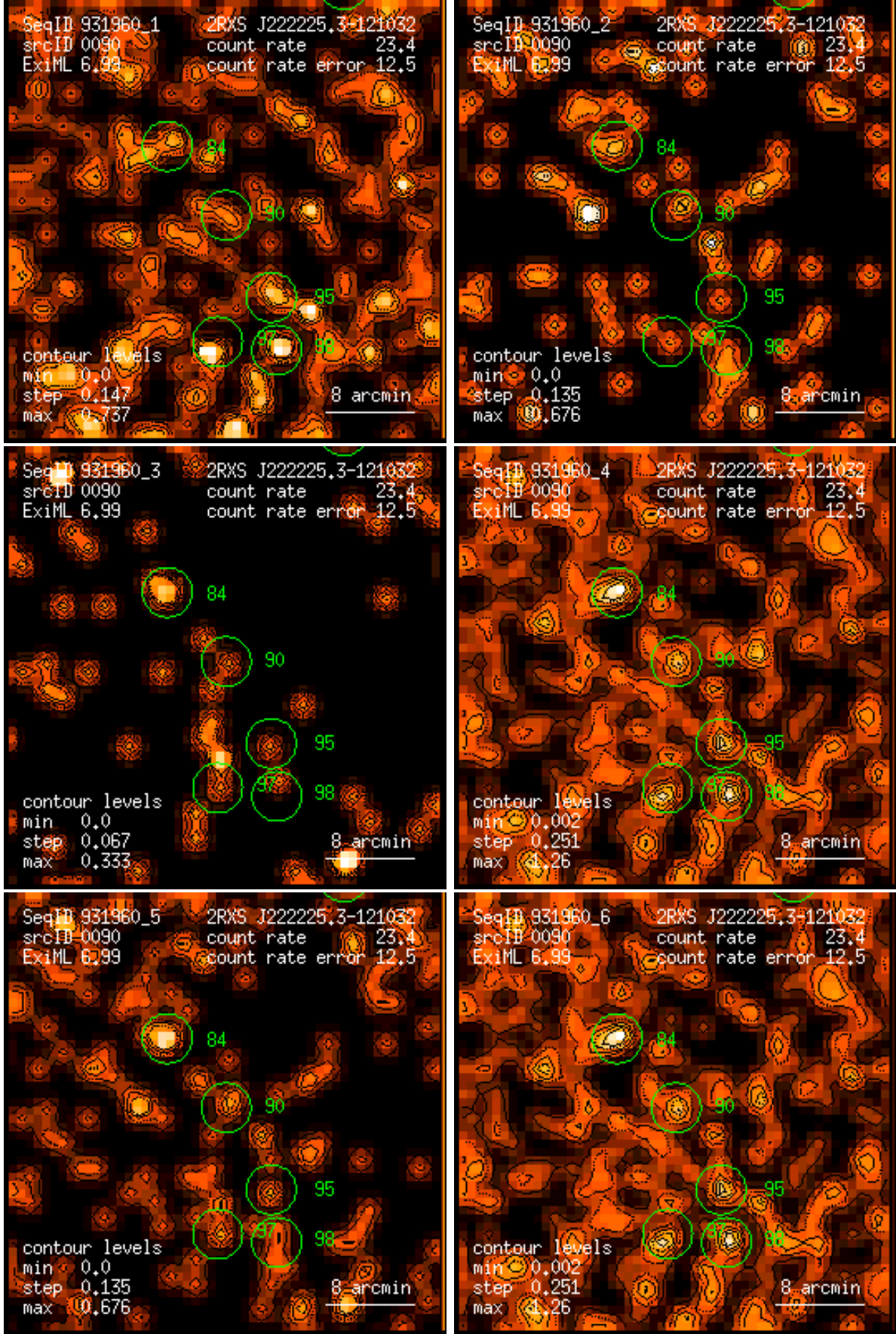
Figure 90: RASS 931960: detection 0090: band rate images, Gaussian filter: (1) PSPC channels 11 – 41, (2) 52 – 90, (3) 91 – 201, (4) 11 – 235, (5) 52 – 201, (6) 11 – 201. Broad band rates in counts/ks. Band rate contour levels in counts/ks/arcmin 2 .
