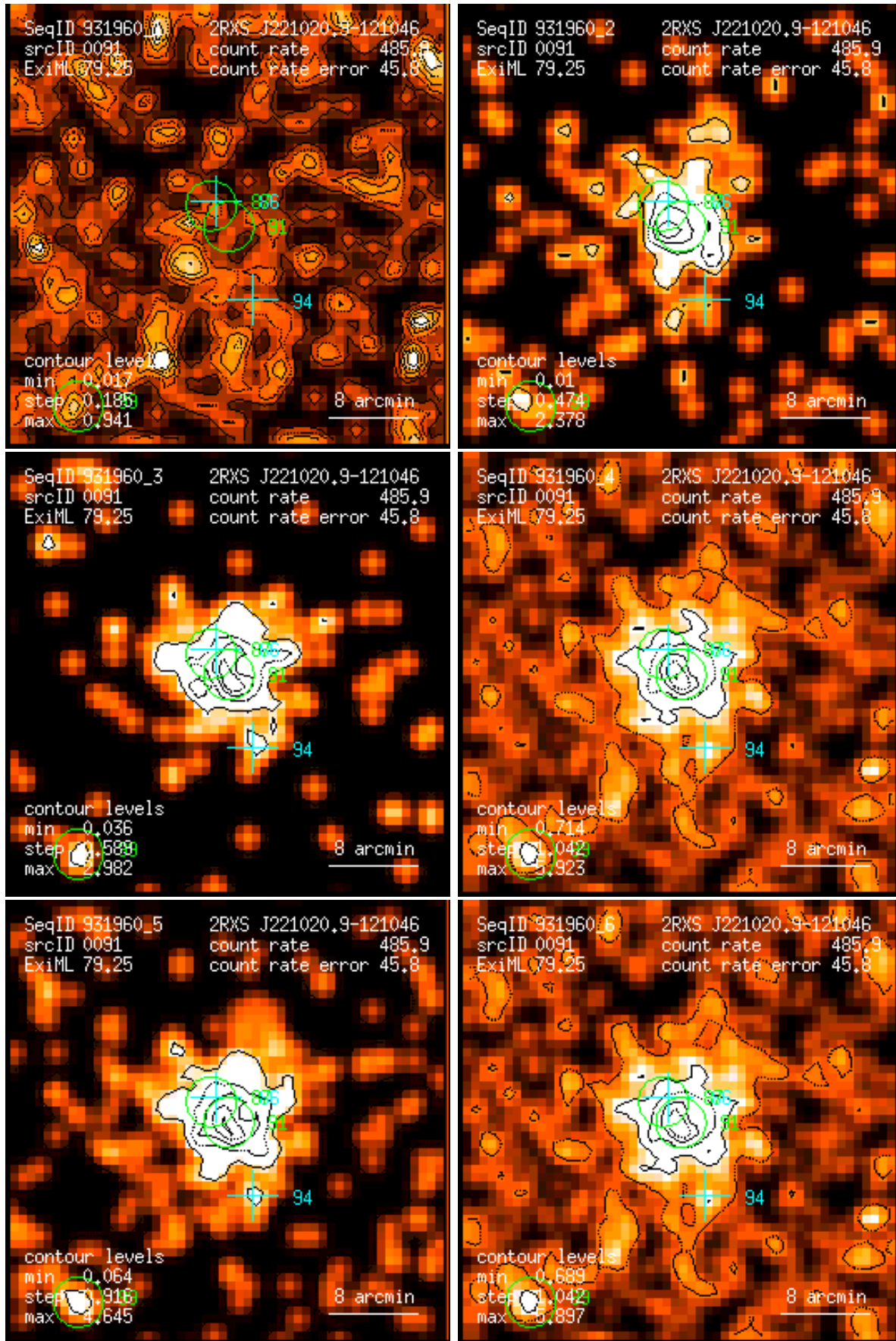
Figure 91: RASS 931960: detection 0091: band rate images, Gaussian filter: (1) PSPC channels 11 – 41, (2) 52 – 90, (3) 91 – 201, (4) 11 – 235, (5) 52 – 201, (6) 11 – 201. Broad band rates in counts/ks. Band rate contour levels in counts/ks/arcmin 2 .
