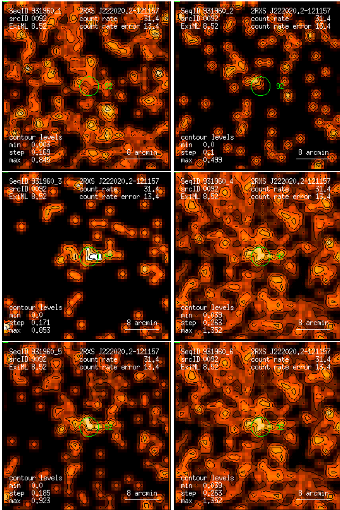
Figure 92: RASS 931960: detection 0092: band rate images, Gaussian filter: (1) PSPC channels 11 – 41, (2) 52 – 90, (3) 91 – 201, (4) 11 – 235, (5) 52 – 201, (6) 11 – 201. Broad band rates in counts/ks. Band rate contour levels in counts/ks/arcmin 2 .
