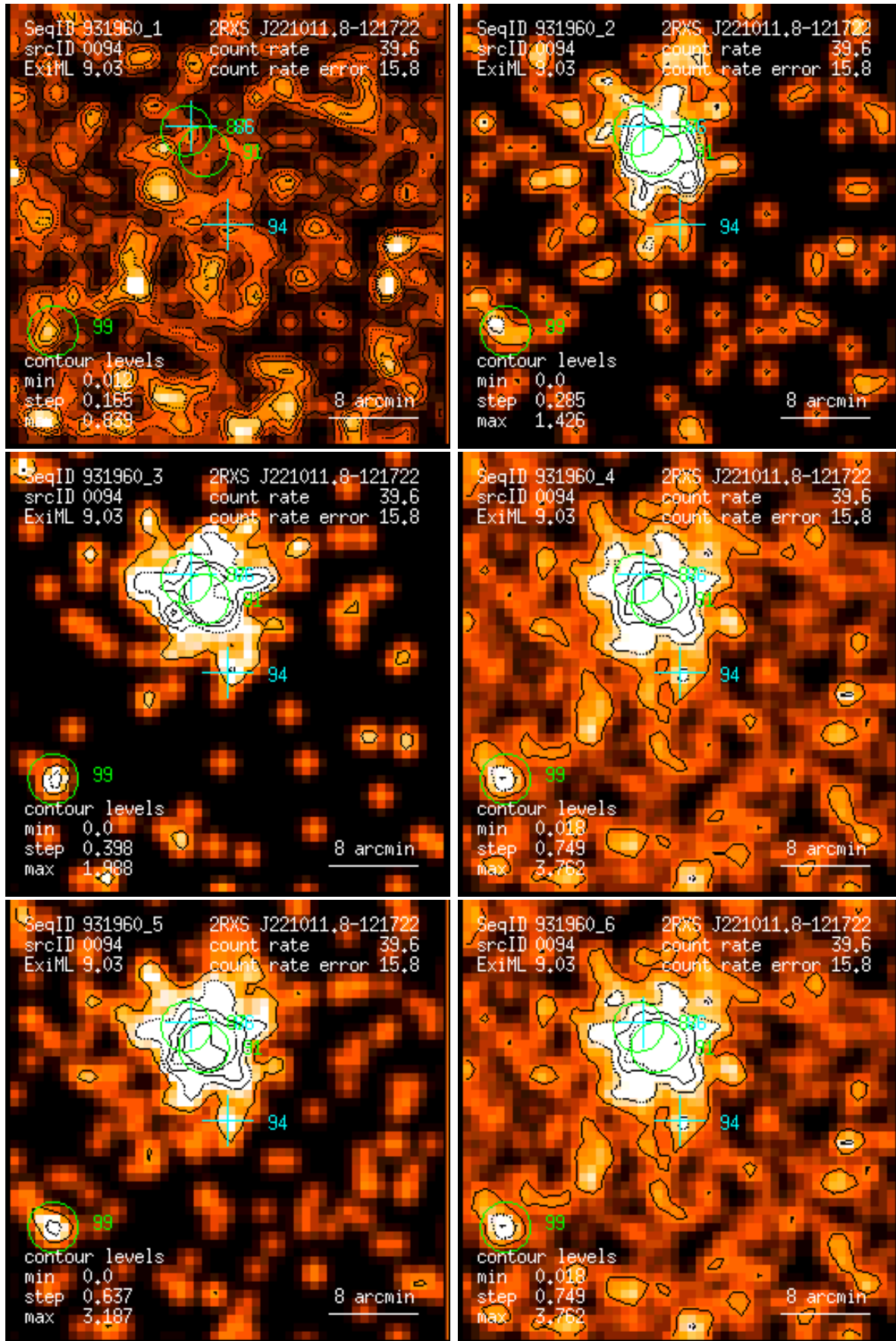
Figure 94: RASS 931960: detection 0094: band rate images, Gaussian filter: (1) PSPC channels 11 – 41, (2) 52 – 90, (3) 91 – 201, (4) 11 – 235, (5) 52 – 201, (6) 11 – 201. Broad band rates in counts/ks. Band rate contour levels in counts/ks/arcmin 2 .
