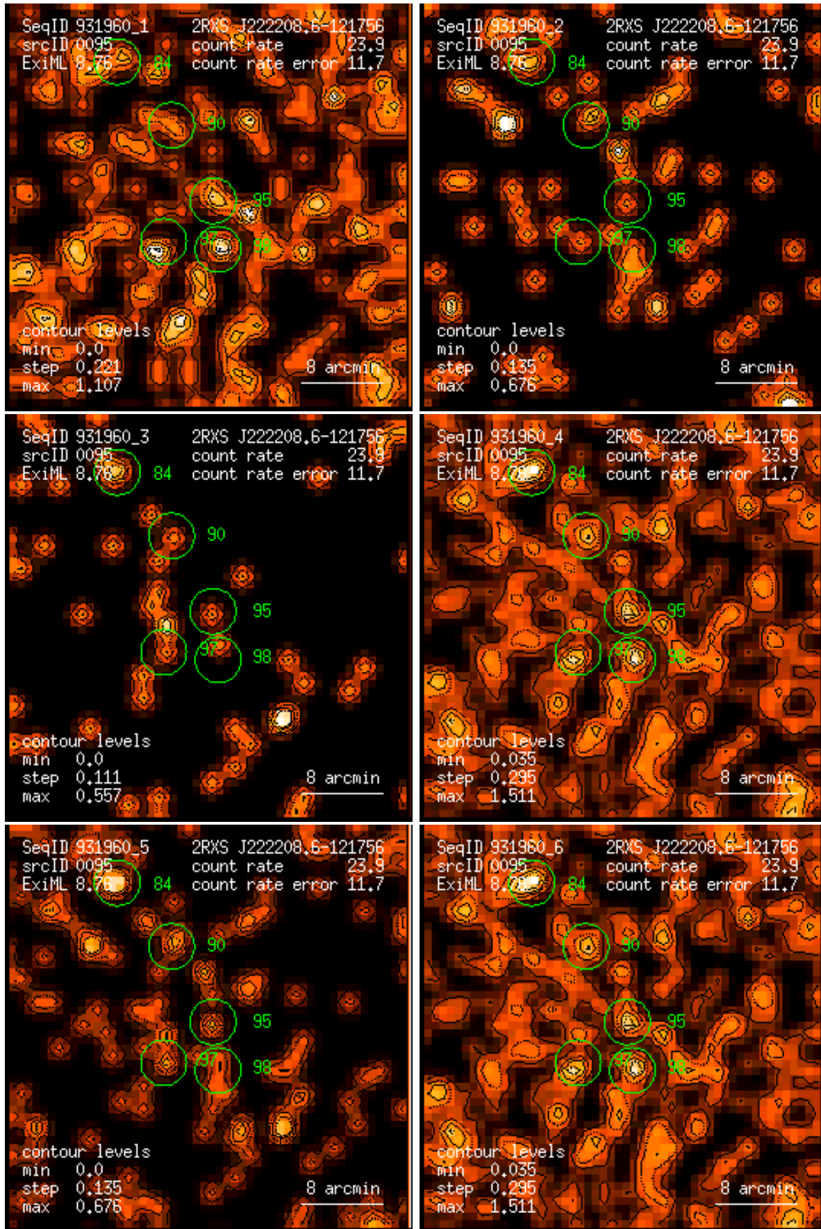
Figure 95: RASS 931960: detection 0095: band rate images, Gaussian filter: (1) PSPC channels 11 – 41, (2) 52 – 90, (3) 91 – 201, (4) 11 – 235, (5) 52 – 201, (6) 11 – 201. Broad band rates in counts/ks. Band rate contour levels in counts/ks/arcmin 2 .
