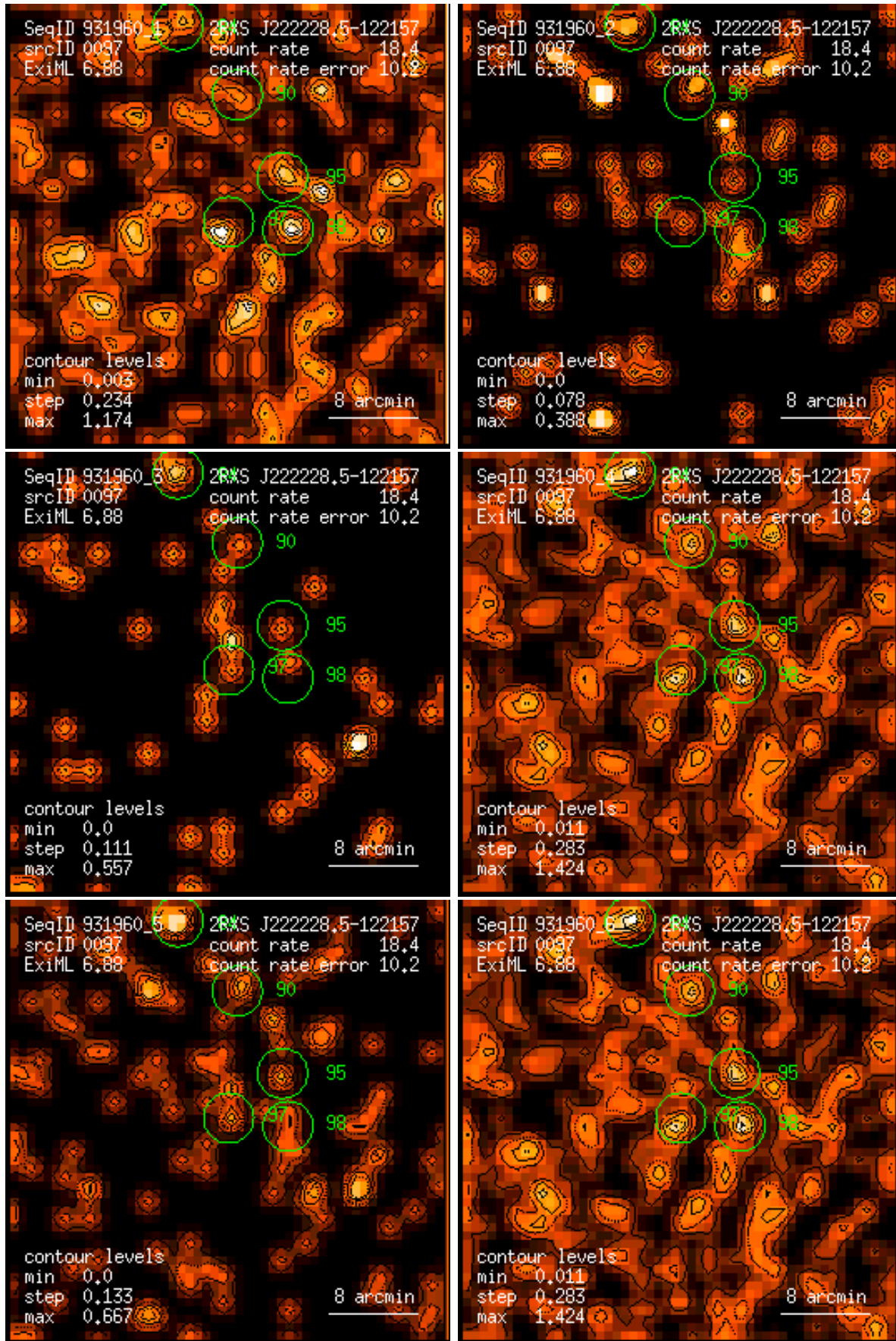
Figure 97: RASS 931960: detection 0097: band rate images, Gaussian filter: (1) PSPC channels 11 – 41, (2) 52 – 90, (3) 91 – 201, (4) 11 – 235, (5) 52 – 201, (6) 11 – 201. Broad band rates in counts/ks. Band rate contour levels in counts/ks/arcmin 2 .
