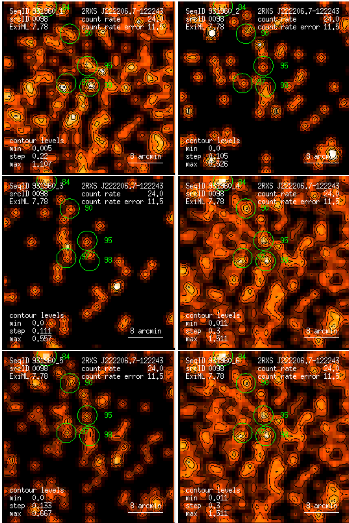
Figure 98: RASS 931960: detection 0098: band rate images, Gaussian filter: (1) PSPC channels 11 – 41, (2) 52 – 90, (3) 91 – 201, (4) 11 – 235, (5) 52 – 201, (6) 11 – 201. Broad band rates in counts/ks. Band rate contour levels in counts/ks/arcmin 2 .
