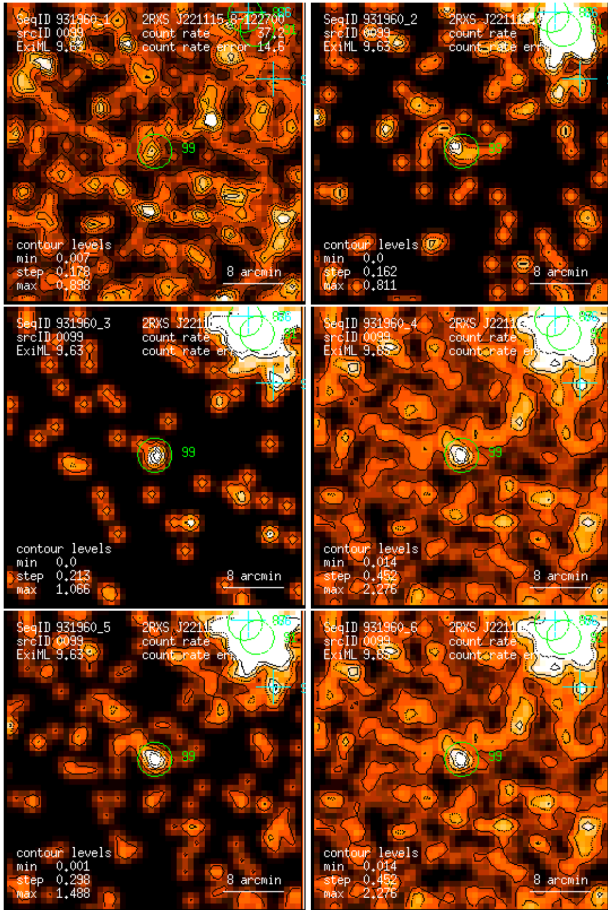
Figure 99: RASS 931960: detection 0099: band rate images, Gaussian filter: (1) PSPC channels 11 – 41, (2) 52 – 90, (3) 91 – 201, (4) 11 – 235, (5) 52 – 201, (6) 11 – 201. Broad band rates in counts/ks. Band rate contour levels in counts/ks/arcmin 2 .
