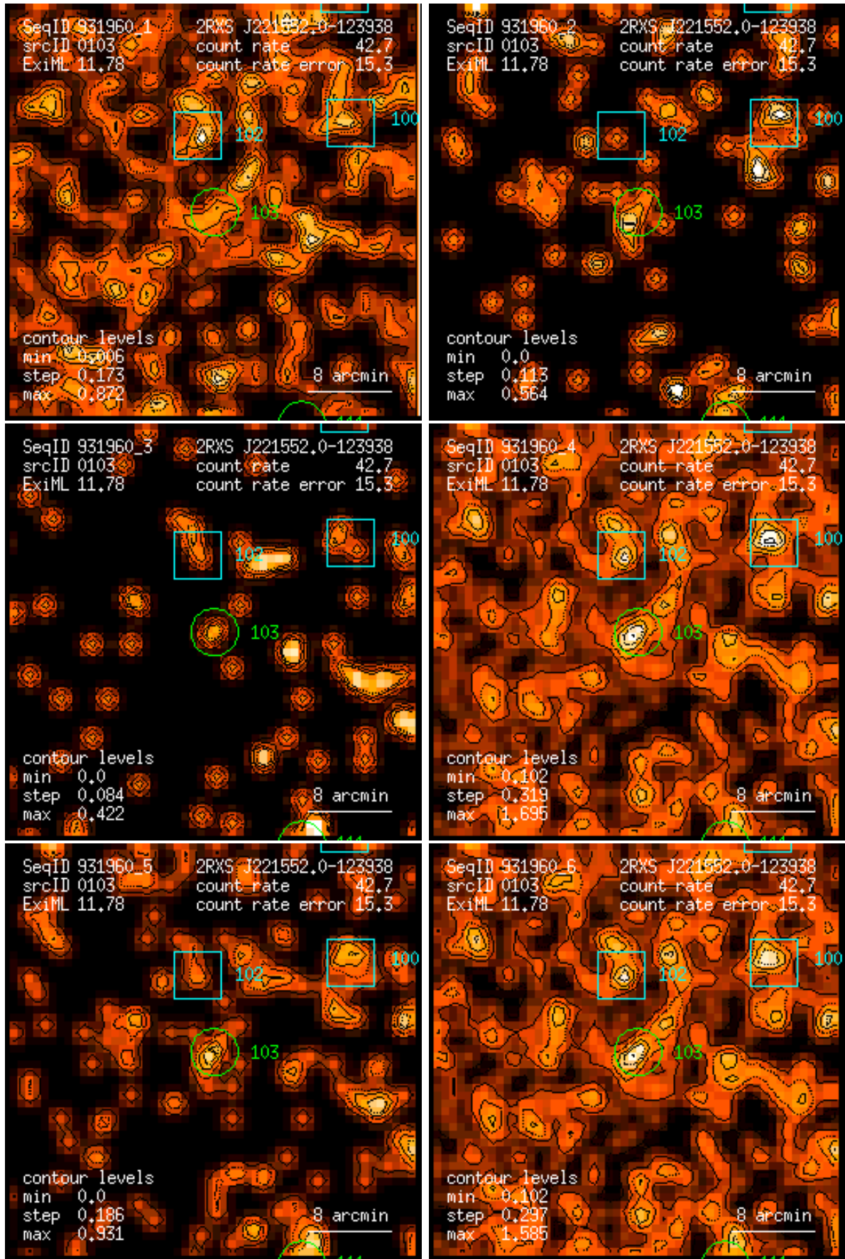
Figure 103: RASS 931960: detection 0103: band rate images, Gaussian filter: (1) PSPC channels 11 – 41, (2) 52 – 90, (3) 91 – 201, (4) 11 – 235, (5) 52 – 201, (6) 11 – 201. Broad band rates in counts/ks. Band rate contour levels in counts/ks/arcmin 2 .
