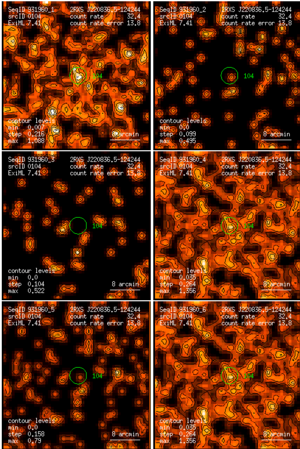
Figure 104: RASS 931960: detection 0104: band rate images, Gaussian filter: (1) PSPC channels 11 – 41, (2) 52 – 90, (3) 91 – 201, (4) 11 – 235, (5) 52 – 201, (6) 11 – 201. Broad band rates in counts/ks. Band rate contour levels in counts/ks/arcmin 2 .
